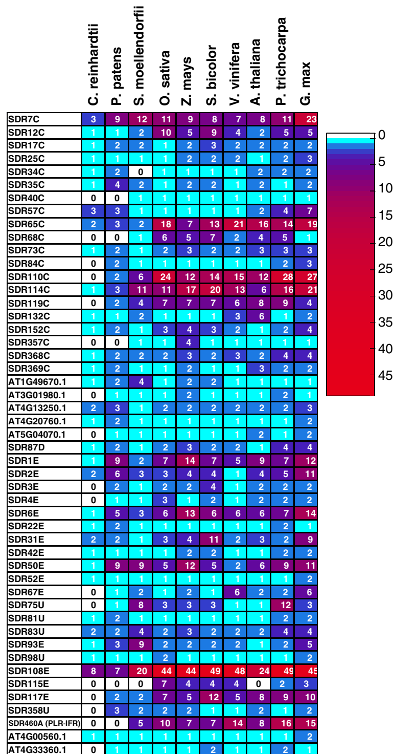
Figure 2 Distribution of the SDR families in the analyzed plant genomes represented as a heat map. The heat map was built on a distribution matrix deduced from the inventory classification shown in Additional file 2: Table S2. The blue to red color gradient reflects the number of SDR listed in each family in the different genomes; the absence of family is indicated with a white square. The names of the families were deduced from the 'SDR Nomenclature Initiative' HMMs or by a representative gene accession for orphan families not recognized by a specific HMM.
