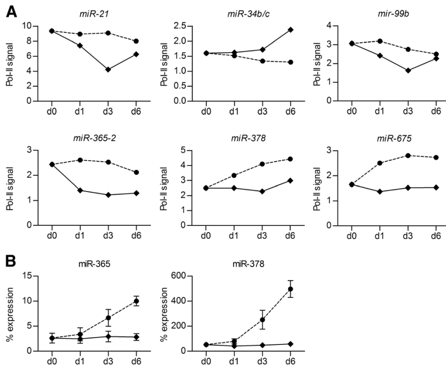
Figure 1 C2C12 lineage-specific miRNA expression. C2C12 cells were treated with (diamonds) or without (circles) 300 ng/ml BMP2 for 6 days, during which chromatin and RNA were harvested in parallel at d0, d1, d3 and d6. A) Pol-II enrichment [27] at regions associated with miRNA genes miR-21 (RefSeq Accession NR_029738; enriched region from -1492 to +1661 bp), miR-34b/c (RefSeq Accessions NR_029655 and NR_029654; enriched regions from -287 to +236 bp ( miR-34b ) and -822 to -299 bp ( miR-34c )), miR-99b (RefSeq Accession NR_029536; enriched region from -1113 to -399 bp), miR-365-2 (RefSeq Accession NR_029959; enriched region from +187 to +1282 bp), miR-378 (RefSeq Accession NR_029879.1; enriched region from -2068 to -130 bp) and miR-675 (RefSeq Accession NR_030416.1; enriched region from -1055 to -235 bp) as determined by Pol-II ChIP-on-chip analysis of single biological samples [27]. B) Mature miRNA levels of miR-365 (3p) and miR-378 (3p) as determined by real-time PCR and expressed as a percentage of the control small, non-coding RNA snoRNA202 . The mean values \pm SD from duplicate measurements are shown for all data points.
