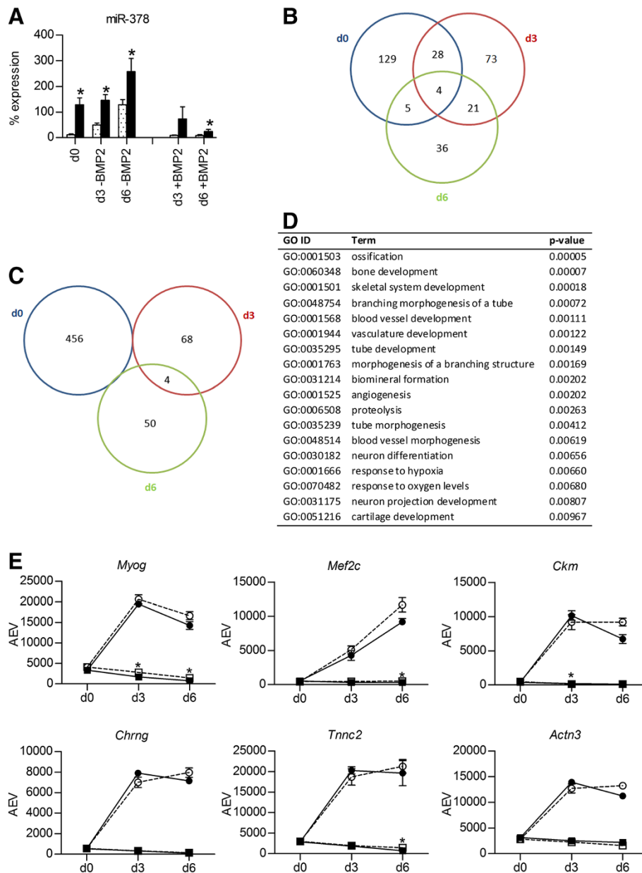
Figure 2 Effect of miR-378 overexpression on C2C12 muscle transcription program. A) Mature miR-378 levels in C2C12-pMirn0 (light bars) and C2C12-pMirn378 (dark bars) cells at indicated time points during treatment with or without 300 ng/ml BMP2. MiR-378 levels are expressed as a percentage of the control small, non-coding RNA snoRNA202 . Mean values \pm SD of three biological replicates, whereby each measurement was made in duplicate, are shown. * p < 0.05 when compared to the C2C12-pMirn0 sample at the same time point and treatment. B-C) Venn diagrams representing the number of probes on the microarray that are significantly lower ( B ) or higher ( C ) expressed in C2C12-pMirn378 cells than in control C2C12-pMirn0 cells at each time point during differentiation in the absence of BMP2. D) Enriched ( p < 0.01 ) GO terms within the set of probes that are significantly lower expressed in C2C12-pMirn378 versus C2C12-pMirn0 cells at at least two consecutive time points during differentiation in the absence of BMP2. E) mRNA expression profiles of the muscle transcription factors myogenin ( Myog ; 1419391_at) and myocyte enhancer factor 2C ( Mef2c ; 1421027_a_at) and other muscle marker genes muscle creatine kinase ( Ckm ; 1417614_at), the acetylcholine receptor subunit gamma ( Chrn3 ; 1449532_at) and the sarcomeric genes fast troponin C2 ( Tnnc2 ; 1417464_at) and actinin alpha 3 ( Actn3 ; 1418677_at) at indicated time points during differentiation of C2C12-pMirn0 (light bullets) and C2C12-pMirn378 (dark bullets) cells treated with (squares) or without (circles) 300 ng/ml BMP2 as revealed from microarray analysis. Mean expression values \pm SD from triplicate microarray experiments are shown for all data points. When the error bar is not visible, the SD falls within the printed data point. All SD values are, however, listed in Additional file 2. AEV = average expression value; *significantly different expression in C2C12-pMirn378 compared to control C2C12-pMirn0 at the same time point and treatment.
