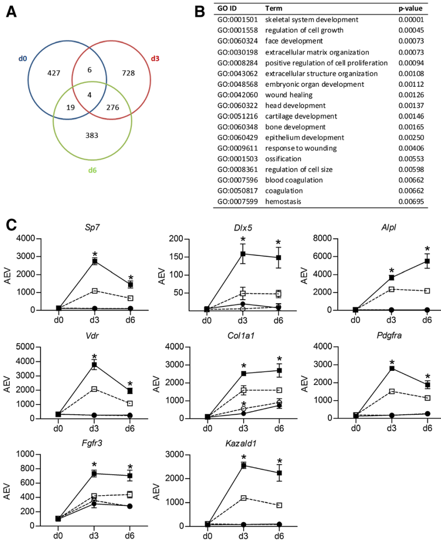
Figure 4 Effect of miR-378 overexpression on C2C12 bone transcription program: upregulation. A) Venn diagram representing the number of probes on the microarray that are significantly (as defined in Methods) higher expressed in C2C12-pMirn378 cells than in control C2C12-pMirn0 cells at each time point during differentiation in the presence of 300 ng/ml BMP2. B) Enriched ( p < 0.01 ) GO terms (in biological processes category) within the set of probes that are significantly higher expressed in C2C12-pMirn378 versus C2C12-pMirn0 cells at at least two consecutive time points during differentiation in the presence of 300 ng/ml BMP2. C) Microarray profiles of bone markers Sp7 transcription factor 7 ( Sp7 ; 1418425_at), distal-less homeobox 5 ( Dlx5 ; 1449863_a_at), alkaline phosphatase ( Alpl ; 1423611_at), vitamin D receptor ( Vdr ; 1418175_at), collagen type I alpha 1 ( Col1a1 ; 1423669_at), platelet derived growth factor receptor alpha polypeptide ( Pdgfra ; 1421917_at), fibroblast growth factor receptor 3 ( Fgfr3 ; 1421841_at) and Kazal-type serine peptidase inhibitor domain 1 ( Kazald1 ; 1436528_at) at indicated time points during differentiation of C2C12-pMirn0 (light bullets) and C2C12-pMirn378 (dark bullets) cells treated with (squares) or without (circles) 300 ng/ml BMP2 as revealed from microarray analysis. Mean expression values \pm SD from triplicate microarray experiments are shown for all data points. When the error bar is not visible, the SD falls within the printed data point. All SD values are, however, listed in Additional file 2. AEV = average expression value; *significantly different expression in C2C12-pMirn378 compared to control C2C12-pMirn0 at the same time point and treatment (see Methods for definition).
