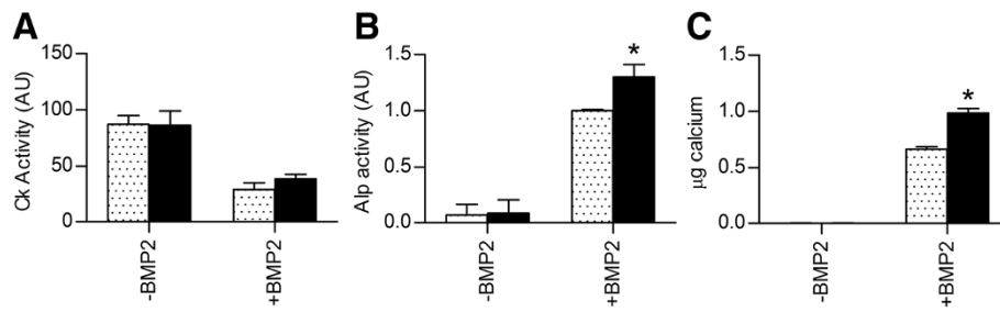
Figure 5 Effect of miR-378 overexpression on C2C12 differentiation. A-C) Creatine kinase (A) and Alp (B) activity in and calcium deposition (C) by C2C12-pMirn0 (light bars) and C2C12-pMirn378 (dark bars) cells after 6 (A-B) or 10 (C) days of culture in the presence or absence of 300 ng/ml BMP2. A) The mean values \pm SD of two biological replicates, whereby each measurement was made in duplicate, are shown. B) Mean values \pm SD of three independent experiments with biological duplicates each. For each independent experiment, Alp activity values were normalized to the average of the C2C12-pMirn0 samples treated with BMP2. C) Data shows calcium deposition in 24-well plates and is representative of 2 independent experiments. Mean values \pm SD of two biological replicates in one experiment, whereby each measurement was made in duplicate, are shown. * p < 0.05 when compared to the C2C12-pMirn0 sample with the same treatment. AU: arbitrary units.
