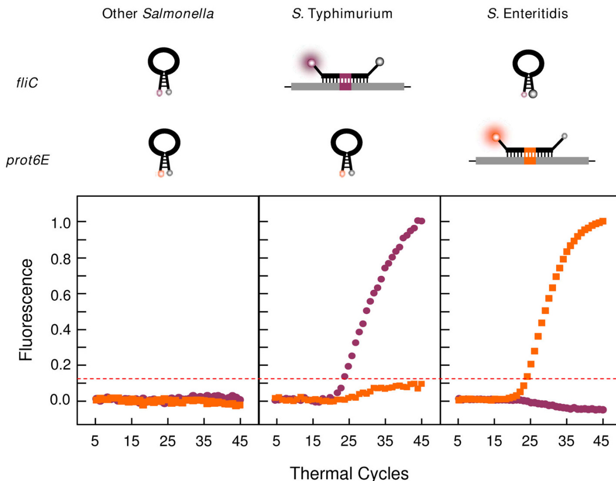
Figure 4 Schematic real-time PCR results for the second step reaction. Representative real-time PCR results as established by the second step multiplex reaction (described in Materials and Methods). The plots show average normalised linear amplification of representative samples shown for demonstration of typical results obtained from S. Typhimurium , S. Enteritidis and other Salmonella samples. With DNA from S. Typhimurium strains, only fliC -specific, HEX-labelled molecular beacons hybridise to the amplicons, generating pink fluorescence, whereas the prot6E -specific, TET-labelled molecular beacons retain their stem-and-loop structure and cannot produce an orange fluorescent signal. With DNA from S. Enteritidis strains, the prot6E -specific, TET-labelled molecular beacons hybridise to their target amplicons and produce an orange fluorescent signal, whereas the fliC -specific, HEX-labelled molecular beacons remain dark. With DNA from other Salmonella serotypes, no target amplicons are detected and both molecular beacons remain dark. The dashed line on the plots represents the normalised threshold for detection of fluorescence, the baseline above which fluorescence increases significantly on amplification and detection of the target sequence.
