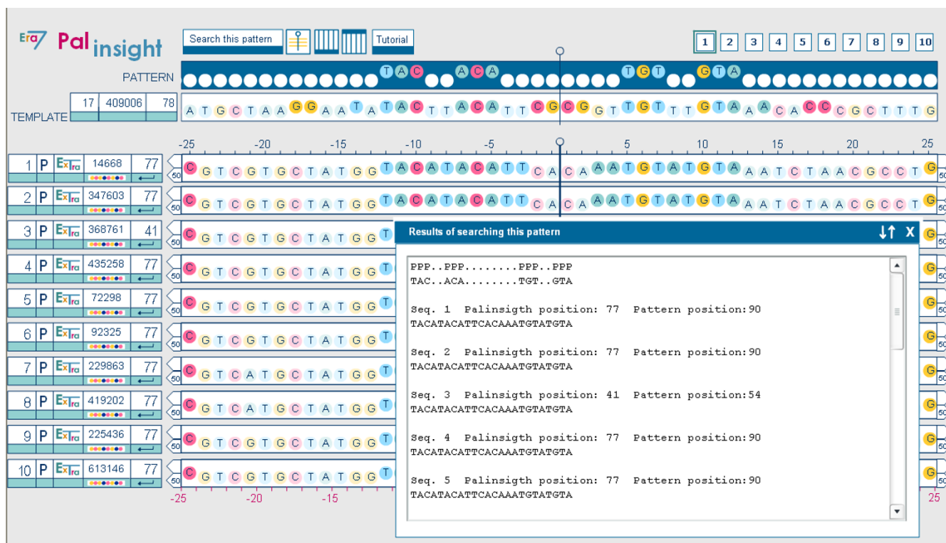
Figure 4 Case study: Palinsight displaying the window of Results of searching the pattern. When we searched for the pattern TAC - -ACA- - -| - - -TGT - -GTA clicking on the "Search this pattern" button we obtained the positions of this motif in the set of selected extragenic sequences. Table 3 is the copy of the complete content of this window.
