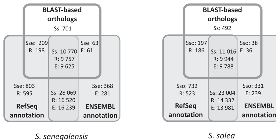
Figure 5 Venn's diagrams reflecting coincidences by Solea species among sole, Blast-based orthologs and transcripts with RefSeq/ ENSEMBL ortholog for zebrafish. Diagrams are comparing the 11,743 Blast-based orthologs with the unique zebrafish RefSeq identifiers in SoleaDB for S. senegalensis (39,851) and S. solea (34,949) and with the unique zebrafish ENSEMBL identifiers in SoleaDB for S. senegalensis (39,270) and S. solea (34,389). Within the Venn's diagrams, the numbers refer to the amount of transcripts in SoleaDB for S. senegalensis (Sse) and S. solea (Sso), the number of transcript in SoleaDB with a zebrafish RefSeq identifier (R) of with a zebrafish ENSEMBL identifier (E).
