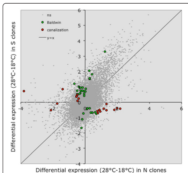
Figure 3 Genes with significant T^*_{\text{geo}} interaction (tested against the pooled random MS; FDR q < 0.05 ), for which the Southern (heat-tolerant) genotypes show greater absolute difference in expression at two temperatures (green symbols, Baldwin effect) or smaller absolute difference in expression at the two temperatures (red symbols, canalization) than the Northern (heat sensitive) genotypes.
