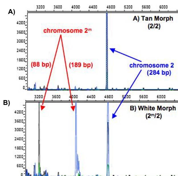
Figure 4 Molecular assay for morph determination. Molecular assay for morph determination in the white-throated sparrow, modified in the Tuttle laboratory for use on automated sequencers from primers described in [50]. Panel A shows a tan morph with a single peak at 284 bp amplified from chromosome 2. Panel B shows a white morph with a band for chromosome 2 (at 284 bp) and two additional bands at 88 bp and 189 bp, which occur when PCR product amplified from chromosome 2 m is digested with restriction endonuclease Dra I. If they occur in nature, we assume that birds homozygous for 2 m ("super whites") would produce a pattern showing only the 88 bp and 189 bp bands. This technique has been verified in adults of known plumage. Values along the y-axis represent the intensity of fluorescence (a.u.), values along the x-axis mark the size of the DNA fragments (a function of time).
