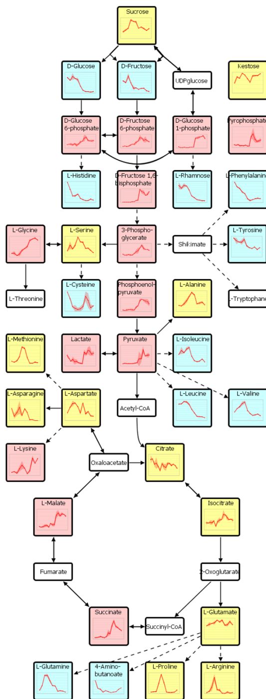
Figure 6 Time series data clustered by self-organizing maps. Wildtype barley ( Hordeum vulgare ) caryopses were harvested every second day over a growth period of about 20 days post anthesis and analyzed for the dynamical changes of several central metabolites. The data set was mapped onto a network that was previously created in VANTED. Each node represents a metabolite, connected by solid and dashed lines that represent single and lumped enzyme reactions, respectively. Data are means of two independent plants, the standard error of the mean (SEM) is shown as a polygon around the line. A self-organizing map algorithm was performed to cluster the metabolites into three groups by similar behavior over time, which is visualized by the background color.
