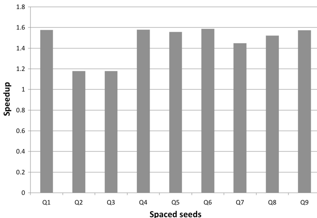
Fig. 1 The speedup of our approach with respect to the standard hashing computation, as a function of the spaced seeds used in our experiments
