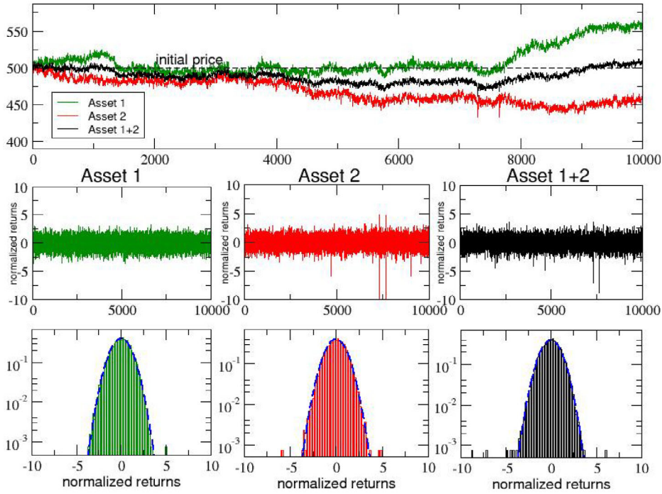
Fig. 3. Top panel: typical time series for the global prices of the two assets ( p_1(t) and p_2(t) ) in absence of correlations ( \delta = 0 ) and for the weighted average price p(t) ( 1 + 2 ). The initial price is also indicated as an horizontal dashed line. Middle panels: normalized returns of the three price series. Bottom right panel: probability density distributions (PDFs) of the normalized returns compared with Gaussian distributions of unitary variance (dashed lines).
