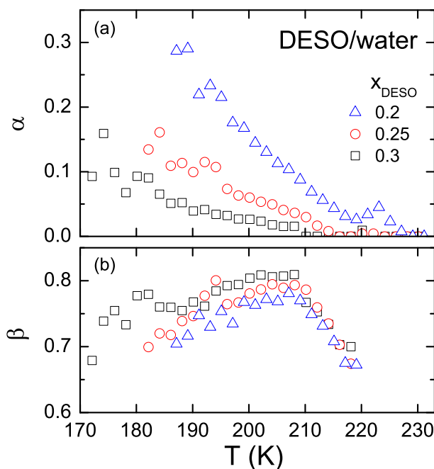
Fig. 4. Temperature dependence of the width parameters \alpha and \beta for DESO/water mixtures obtained from the simultaneous fits of the real and imaginary parts of the complex dielectric permittivity with the HN function, eq. (1).
