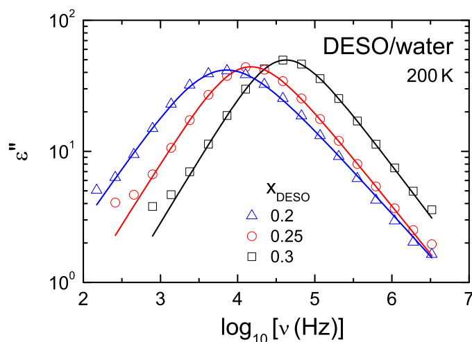
Fig. 3. Comparison of dielectric-loss spectra of DESO/water mixtures at three concentrations ( x_{\text{DESO}} = 0.2, 0.25 and 0.3 ), measured at a temperature of 200 K. The solid lines are fits using the HN function, eq. (1).
