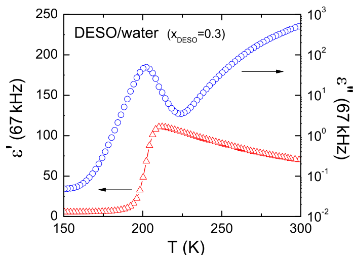
Fig. 1. Temperature variation of the real part \epsilon' and imaginary part \epsilon'' of the complex dielectric permittivity at a frequency of 67 kHz for a DESO/water solution with x_{\text{DESO}} = 0.3 .
