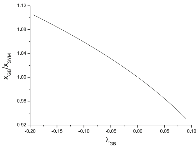
Fig. 3 x_{GB}/x_{SYM} versus \lambda_{GB} . Here we take |\vec{q}| = 0.99\omega
