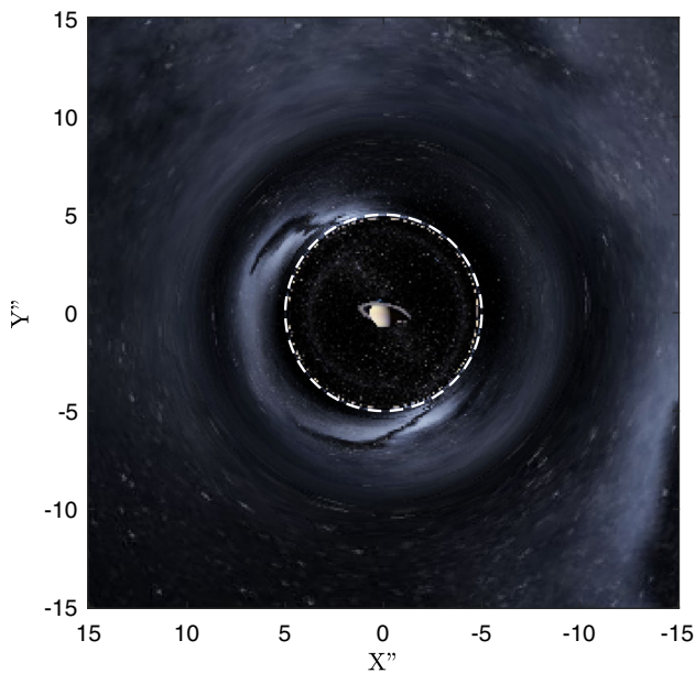
Fig. 8 Apparent image of a Morris and Thorne-like WH in metric theory of gravity [13]. We set b_0 = 5 , r_{\text{skyph}} = 8b_0 (computational domain limit or infinite), \Delta L_p = b_0/50 , and d_{\text{plate}} = 4b_0 . The white dashed circle represents the WH mouth size b_0 . Credits for textures used in this image to [29]
