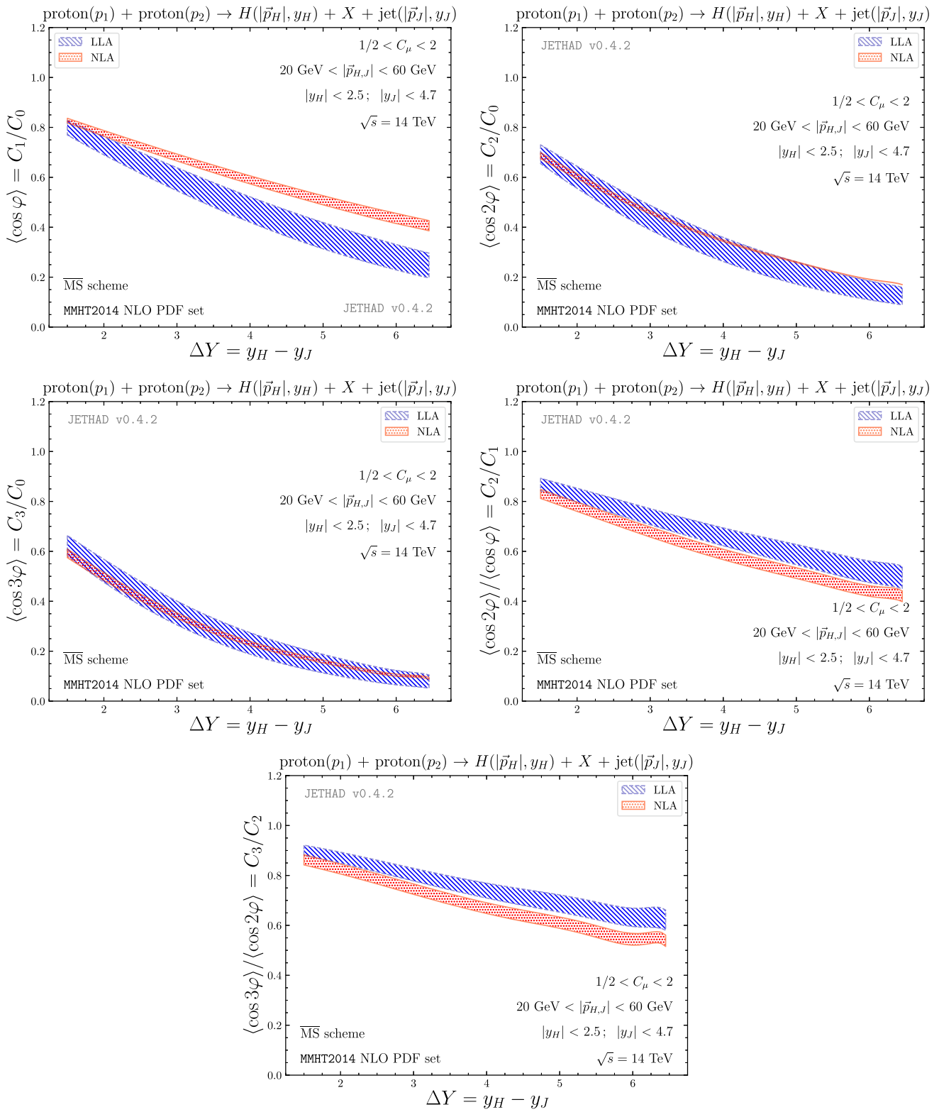
Fig. 5 \Delta Y -dependence of several ratios R_{nm} \equiv C_n/C_m , for the inclusive Higgs-jet hadroproduction in the p_T -symmetric configuration and for \sqrt{s} = 14 TeV. Shaded bands give the combined effect of the scale variation with the uncertainty coming from the phase-space numerical integration
