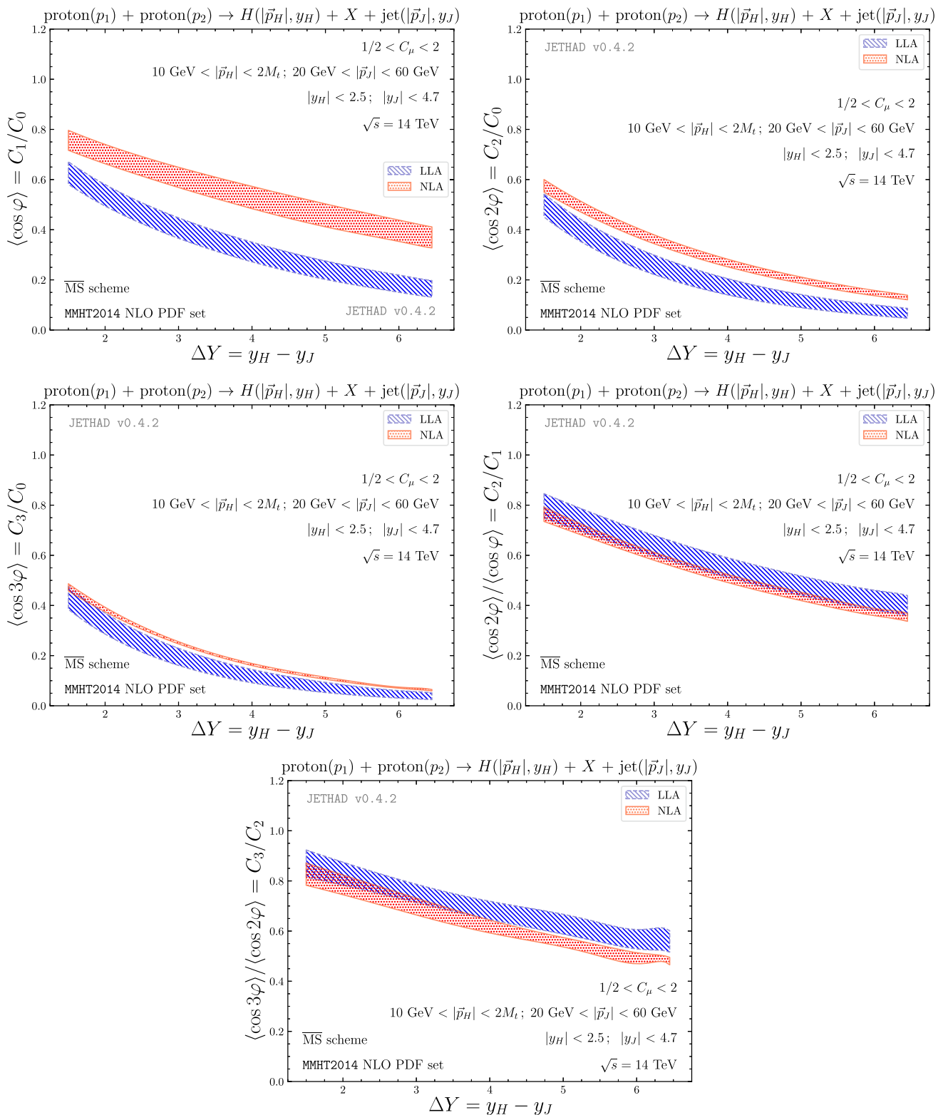
Fig. 6 \Delta Y -dependence of several ratios R_{nm} \equiv C_n/C_m , for the inclusive Higgs-jet hadroproduction in the p_T -asymmetric configuration and for \sqrt{s} = 14 \text{ TeV} . Shaded bands give the combined effect of the scale variation with the uncertainty coming from the phase-space numerical integration
