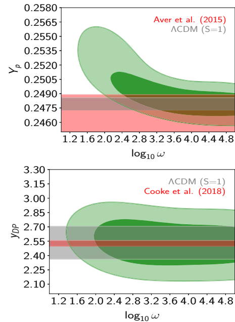
Fig. 6 The 2D constraints on the BBN predicted ^4\text{He} (helium) mass fraction Y_p (top panel) and \text{D} (deuterium) y_{DP} mass fraction (bottom panel) in BD gravity are plotted with 1\sigma (dark green) and 2\sigma (light green) confidence contours. Grey bands are for the SBBN-predicted mass fractions with 1\sigma . Red bands are independent observational estimates with 1\sigma from [157, 158]
