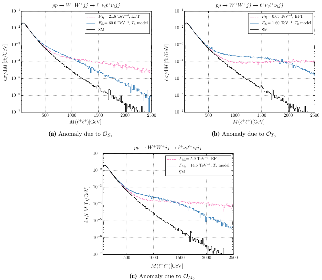
Fig. 5 Differential cross section as a function of the invariant mass m_{\ell\ell} of the charged leptons for pp \rightarrow \ell^+ \nu_\ell \ell^+ \nu_\ell jj X . The solid black line shows the SM, while the dashed pink solid line shows the cross section for the anomalous coupling using the present CMS upper limit.
