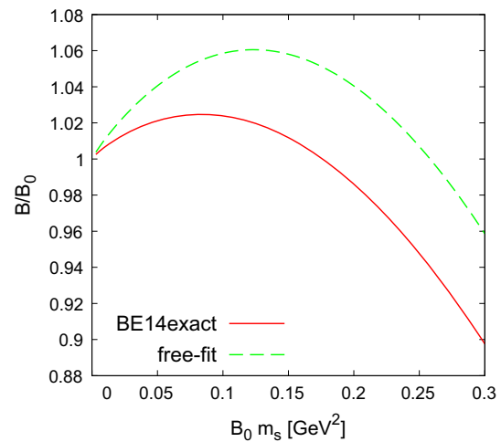
Fig. 5 m_s dependence of M_\pi^2/m_\pi^2 in the chiral limit
