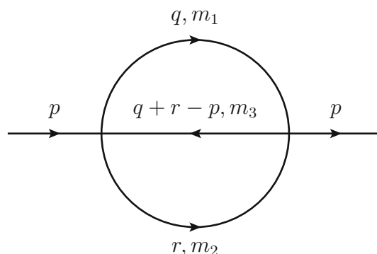
Fig. 1 The two-loop self-energy “sunset” diagram
