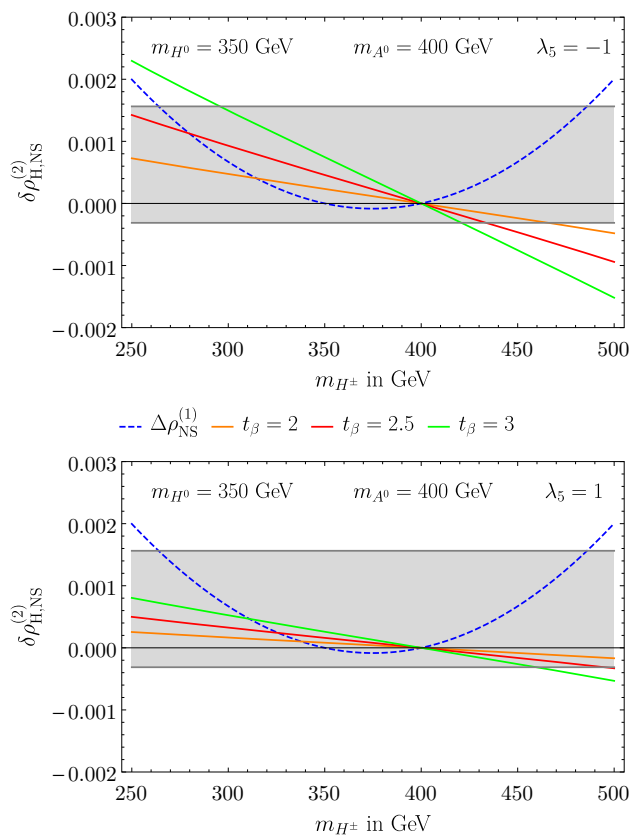
Fig. 13 Effect of mass differences between neutral and charged scalars on \delta\rho_{H,NS}^{(2)} for \lambda_5 = \pm 1 . The neutral masses are fixed at m_{H^0} = 350 GeV and m_{A^0} = 400 GeV. The mass of H^\pm is varied from 250 GeV to 500 GeV. The solid lines represent different values of t_\beta as explained in the legend. The blue dashed line shows the non-standard one-loop correction \Delta\rho_{NS}^{(1)} for comparison. The gray area depicts the bounds from the experimental limits of the T parameter
