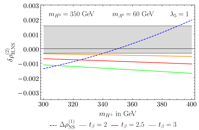
Fig. 17 Results for \delta\rho_{H,\text{NS}}^{(2)} for m_{A^0} = 60 GeV. The mass of H^0 is fixed at 350 GeV. The different solid lines correspond to different values of t_\beta . The non-standard one-loop correction \Delta\rho_{\text{NS}}^{(1)} is shown by the blue dashed line . The gray area corresponds to the bounds from the experimental limits of the T parameter
