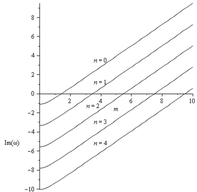
Fig. 1 In this plot we depict the behavior of the QNMs expressed in Eq. (71), with some parameter values, l = 1 and u_+ = \sqrt{5} . We can see that the BH becomes unstable for large values of the mass m
