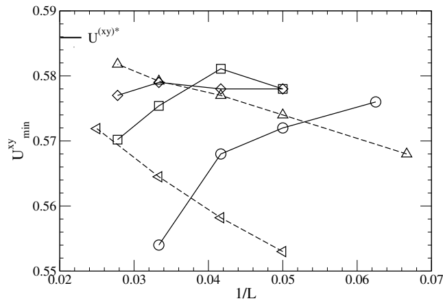
Fig. 7. Minimum of the xy -cumulant U_{min}^{xy} as a function of lattice size L for various temperatures k_B T/J = 1.3 (circles), 1.45 (squares), 1.5 (diamonds), and 1.55 (triangles left) as well as for fixed field H/J = 4.03 (triangles up). The critical cumulant in the XY universality class occurs at U^{(xy)*} \approx 0.586 [45, 46].
