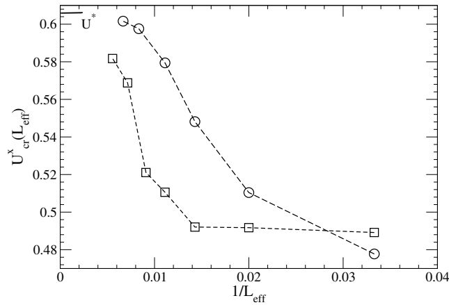
Fig. 3. Finite-size dependence of the crossing points of the longitudinal Binder cumulants U_{\text{cr}}^x(L_{\text{eff}}) at k_B T/J = 0.6 (squares) and 0.7 (circles). The value of the critical cumulant for the Ising case U^* = 0.61069\dots is indicated.
