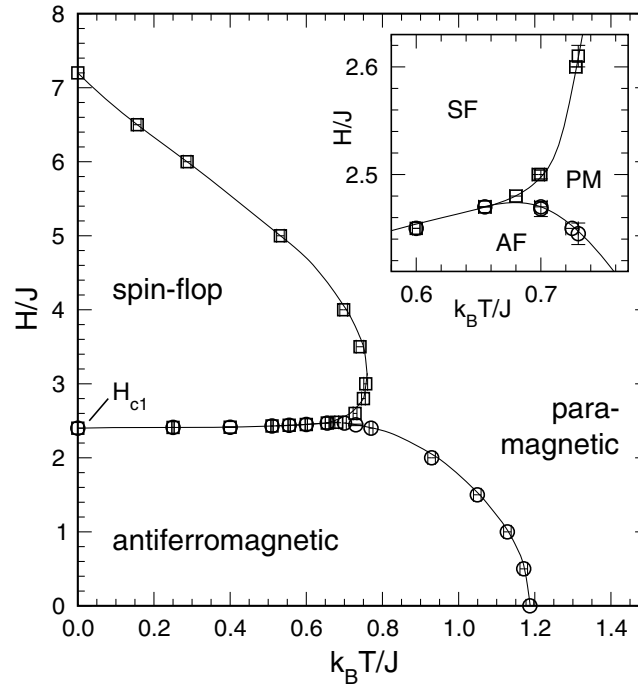
Fig. 2. Phase diagram of the anisotropic XY antiferromagnet on the square lattice with \Delta = 0.8 . From reference [22].
