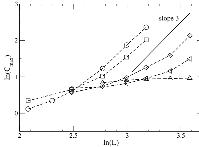
Fig. 5. Maximal specific heat, C_{max} , versus lattice size, L , near the AF-SF transition at k_B T/J = 1.0 (circles), 1.3 (squares), 1.45 (diamonds), 1.50 (triangles left), and 1.55 (triangles up). The straight line corresponds to C_{max} \propto L^3 .
