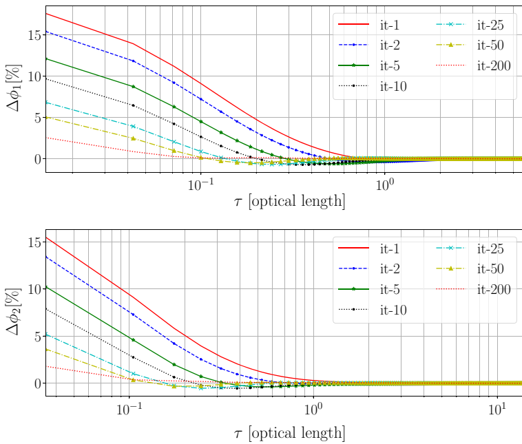
Fig. 9 The spatial flux convergence of the Ronen iterations with respect to the reference S_{16} solution for the left half slab
