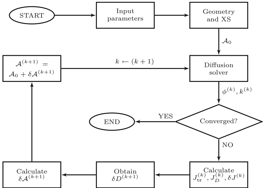
Fig. 3 A flowchart of the Ronen algorithm
