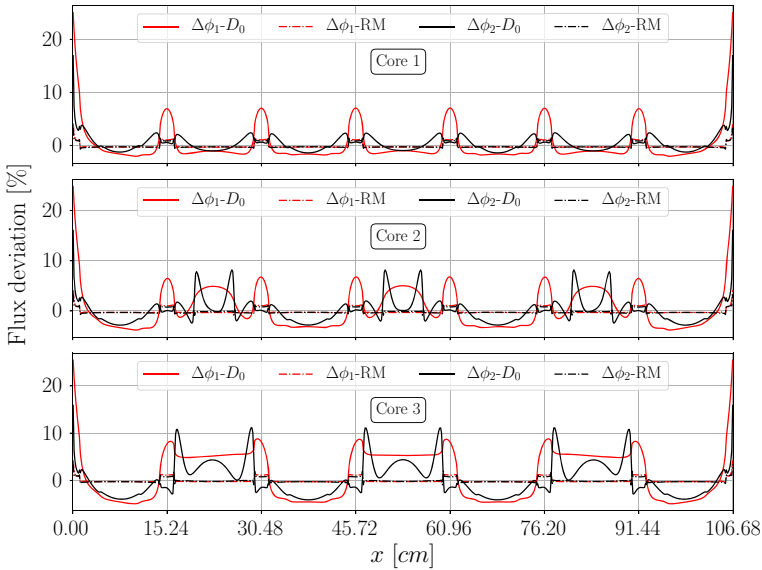
Fig. 12 Fast and thermal flux deviation of standard diffusion ( D_0 ) and Ronen method (RM) with respect to S_{16} reference solutions for each core. Vertical grid lines are located at assemblies interfaces. RM results are for 100 iterations, and the spatial mesh spans 8 nodes in the water and 22 nodes in each fuel element
