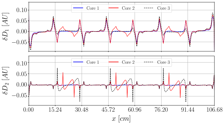
Fig. 13 Behavior of the Ronen method correction factor \delta D along the core, for the fast and thermal fluxes. Vertical grid lines are located at assemblies interfaces, results are for 100 iterations, and the spatial mesh spans 8 nodes in the water and 22 nodes in each fuel element
