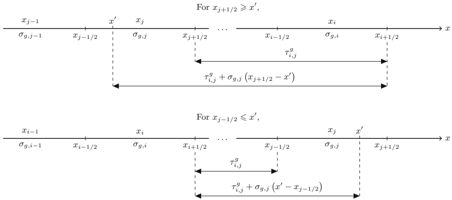
Fig. 2 Notation for numerical evaluation of interface currents by the integral form of the transport equation
