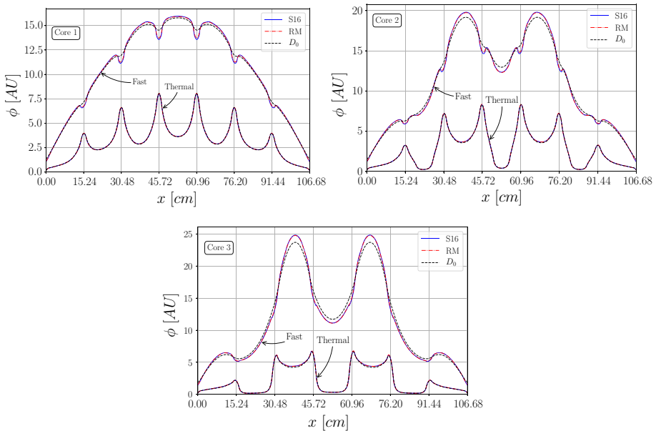
Fig. 11 Fast and thermal flux for each core using standard diffusion ( D_0 ), Ronen method (RM) and S_{16} reference solution. Vertical grid lines are located at assemblies interfaces. RM results are for 100 iterations, and the spatial mesh spans 8 nodes in the water and 22 nodes in each fuel element
