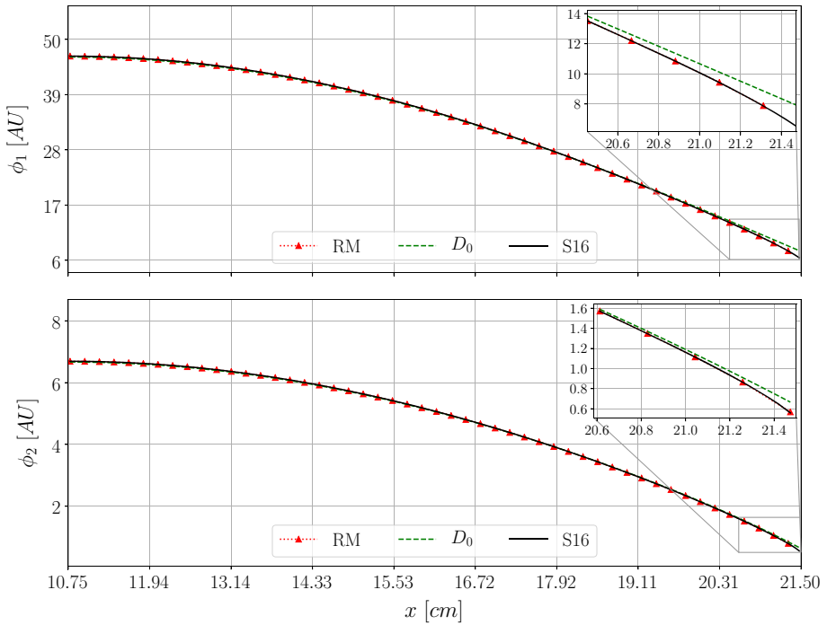
Fig. 4 Comparison of the fluxes as calculated by the reference S_N code, the RM code, and a standard multigroup diffusion without RM correction ( D_0 ). The insets show a zoom-in of the fluxes near the boundary. Results shown here after 250 Ronen iterations
