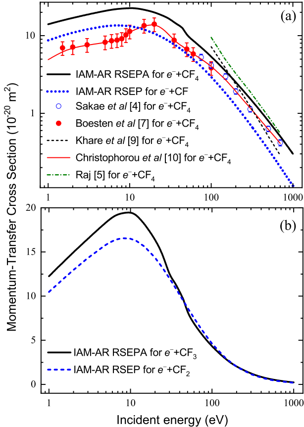
Fig. 2. Momentum-transfer integral cross sections of electron scattering by CF and CF 4 (a) as well as by CF 2 and CF 3 (b) molecules.
