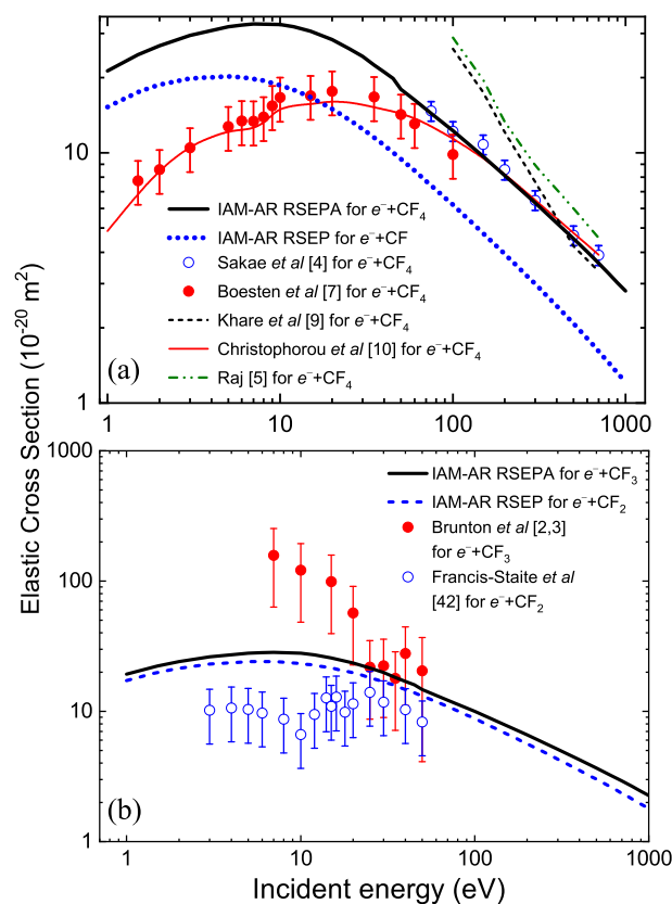
Fig. 1. Elastic integral cross sections of electron scattering by CF and \text{CF}_4 (a) as well as by \text{CF}_2 and \text{CF}_3 (b) molecules.
