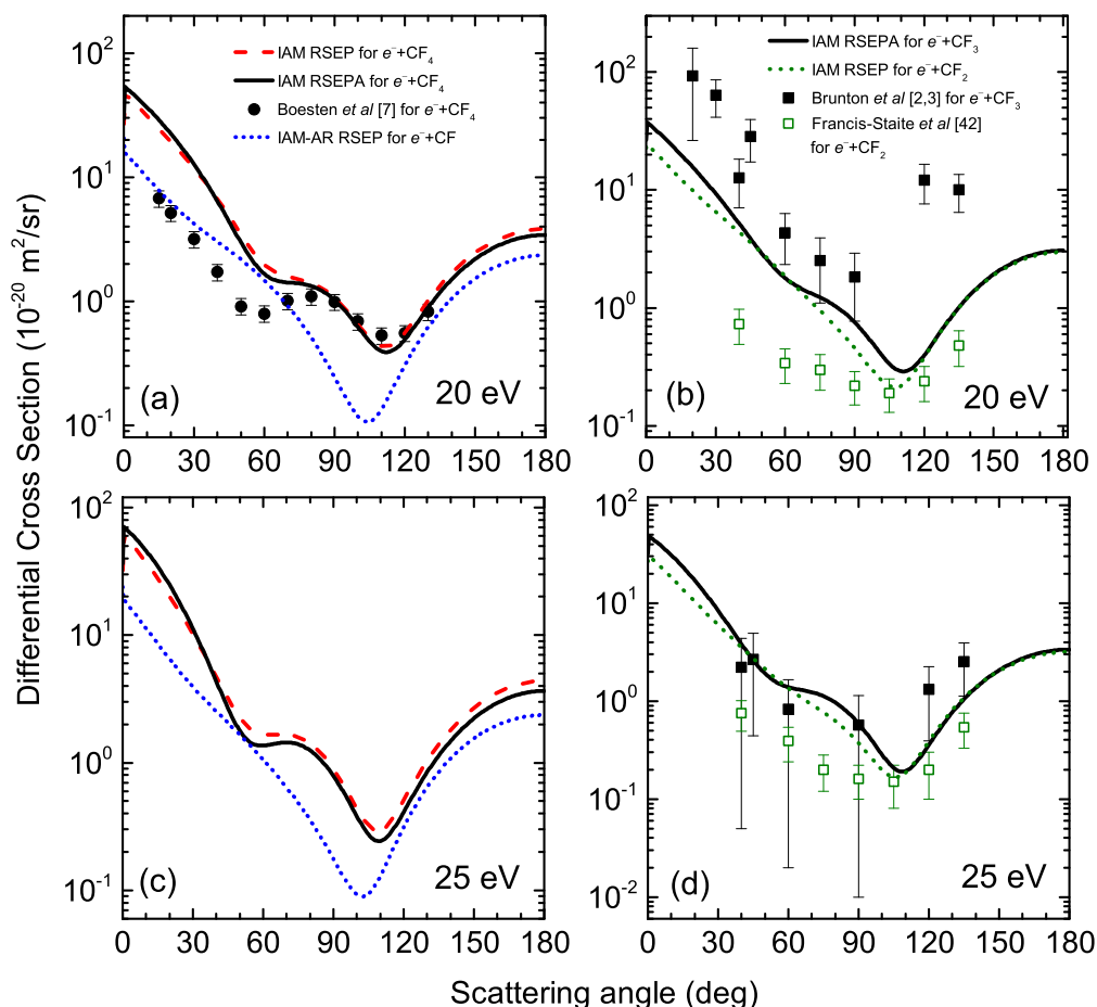
Fig. 4. The angular behaviour of differential cross sections for elastic electron scattering by CF and CF 4 (a,c) and also by CF 2 and CF 3 (b,d) molecules at 20 and 25 eV collision energies.
