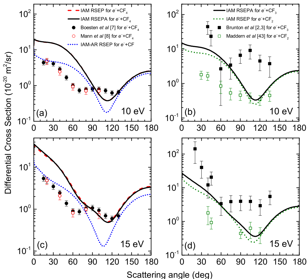
Fig. 3. The angular behaviour of differential cross sections for elastic electron scattering by CF and CF 4 (a,c) and also by CF 2 and CF 3 (b,d) molecules at 10 and 15 eV collision energies.
