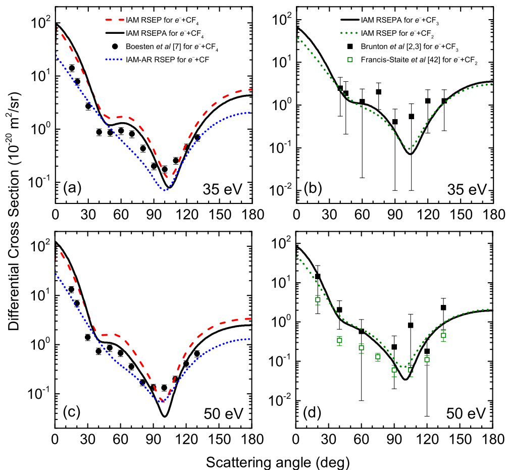
Fig. 5. The angular behaviour of differential cross sections for elastic electron scattering by CF and CF 4 (a,c) and also by CF 2 and CF 3 (b,d) molecules at 35 and 50 eV collision energies.
