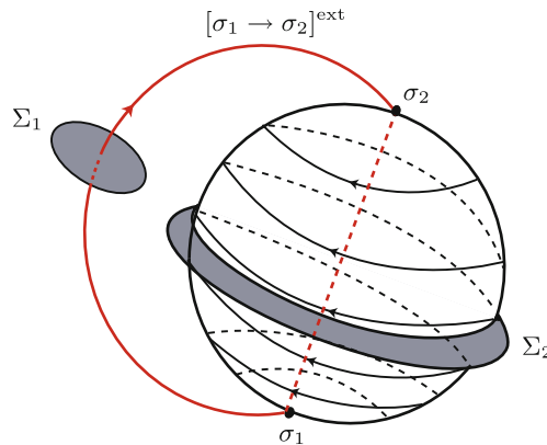
Fig. 3. \Sigma_1 and \Sigma_2 .
