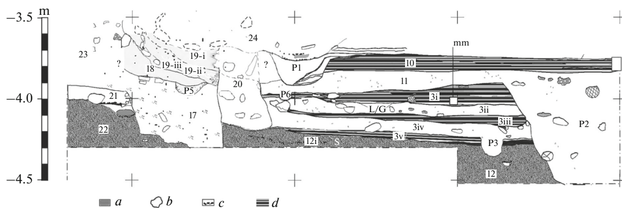
Fig. 2. Tell Körkik Tepe, Epipaleolithic layer in the eastern section of trench 21: thin-layered sediments of dwelling floors (3i, 3iii, 3v, and 10) alternating with the layers of leveled surface (3iv, 3ii, and 11); S—sand; P—pit; mm—loci of sampling for the micro-morphological study; (a) clay; (b) stones; (c) charcoal; and (d) thin-layered sediments.
