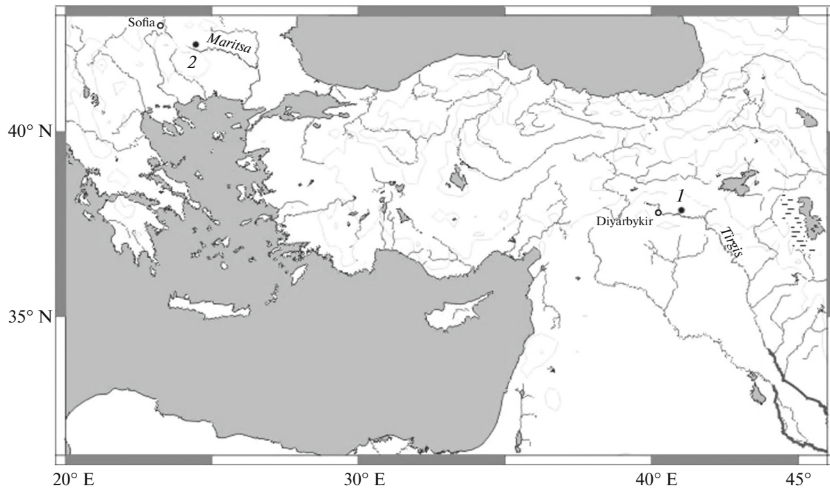
Fig. 1. Location of studied objects: (1) Tell Körтик Tepe and (2) Tell Yunatsite.
