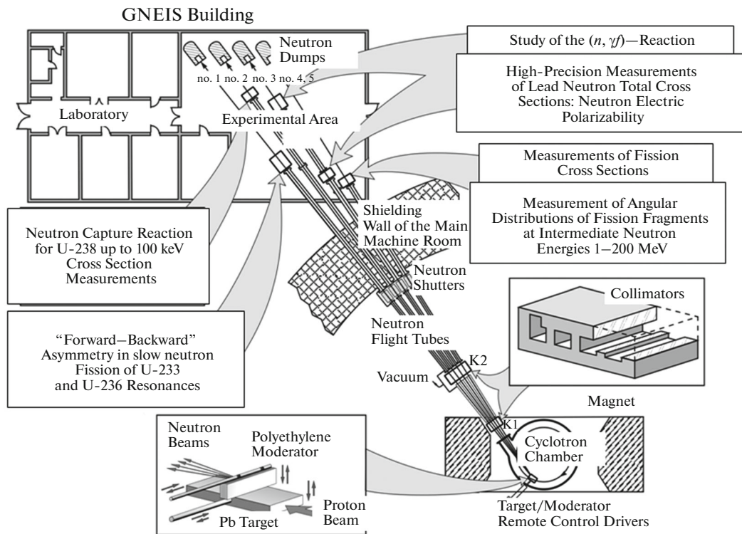
Fig. 1. General layout of the GNEIS facility.
