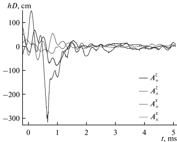
Filtered gravitational wave amplitudes from a 3D full-star quark nova simulation with the bag constant B^{1/4} = 147 MeV (from [38]).
