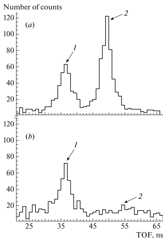
Fig. 3. Time spectra of signals from the gamma-ray detectors: (a) time spectrum recorded by the gamma-ray detector no. 1, which is positioned at an angle of 1^\circ with respect to one of the tagged-neutron beams, and (b) analogous spectrum from detector no. 9, which is positioned at an angle of 130^\circ with respect to the same beam. Peaks 1 and 2 are associated with gamma rays and neutrons, respectively.
