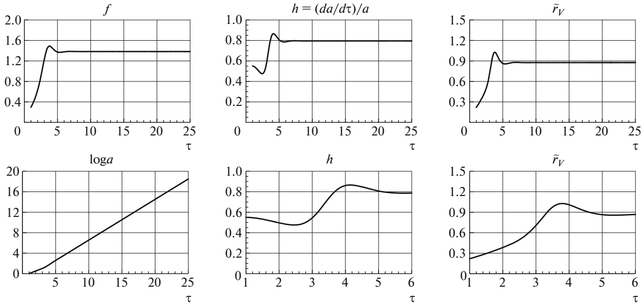
Fig. 1. Numerical solution for the evolution of the universe after a cosmic catastrophe, neglecting dissipation. The model parameters of the ODEs (17) with auxiliary functions (18) are (w_M, \gamma_f, \gamma_h) = (1/3, 0, 0) and the boundary conditions at \tau = 1 are \{a(1), h(1), \dot{h}(1), f(1), r_M(1)\} = \{1, 0.55, 0, 0.2953, 0\} . With these parameters and boundary conditions, the matter energy density vanishes exactly, r_M(\tau) = 0 for \tau \geq 1 .
