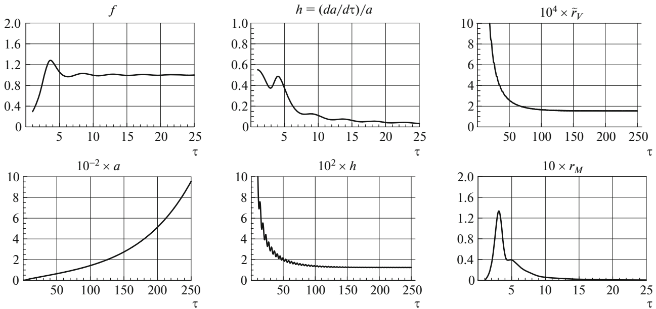
Fig. 2. Numerical solution for the evolution of the universe after a cosmic catastrophe, taking into account dissipation, which leads to energy exchange between vacuum and matter. The model parameters of the ODEs (17) are (w_M, \gamma_f, \gamma_h) = (1/3, 1, 1) . The boundary conditions at \tau = 1 are the same as in Fig. 1, \{a(1), h(1), \dot{h}(1), f(1), r_M(1)\} = \{1, 0.55, 0, 0.2953, 0\} .
