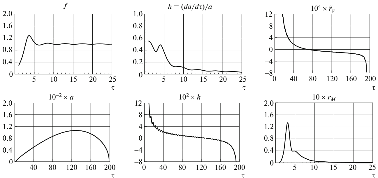
Fig. 3. Numerical solution of the ODEs (17), taking into account dissipation. The model parameters are the same as in Fig. 2, (w_M, \gamma_f, \gamma_h) = (1/3, 1, 1) , but the boundary conditions at \tau = 1 are different, \{a(1), h(1), \dot{h}(1), f(1), r_M(1)\} = \{1, 0.55, 0, 0.2952, 0\} . The scale factor a(\tau) of the numerical solution drops to a value O(10) at \tau \approx 198 .
