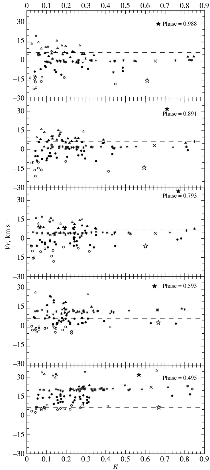
Fig. 8. Radial velocity V_r measured from the cores of the metal absorption lines, their blue (B1, B2) and red (R1, R2) components, the H\alpha line, and its B and R components versus line depth. The asterisks are the metal lines, the filled circles are the B1 components, the open circles are the B2 components, the filled triangles are the R1 components, the open triangles are the R2 components, the cross is the H\alpha center, the filled five-point star is the R component, and the open five-point star is the B component. The \langle V_r \rangle estimate is indicated by the dotted line.
