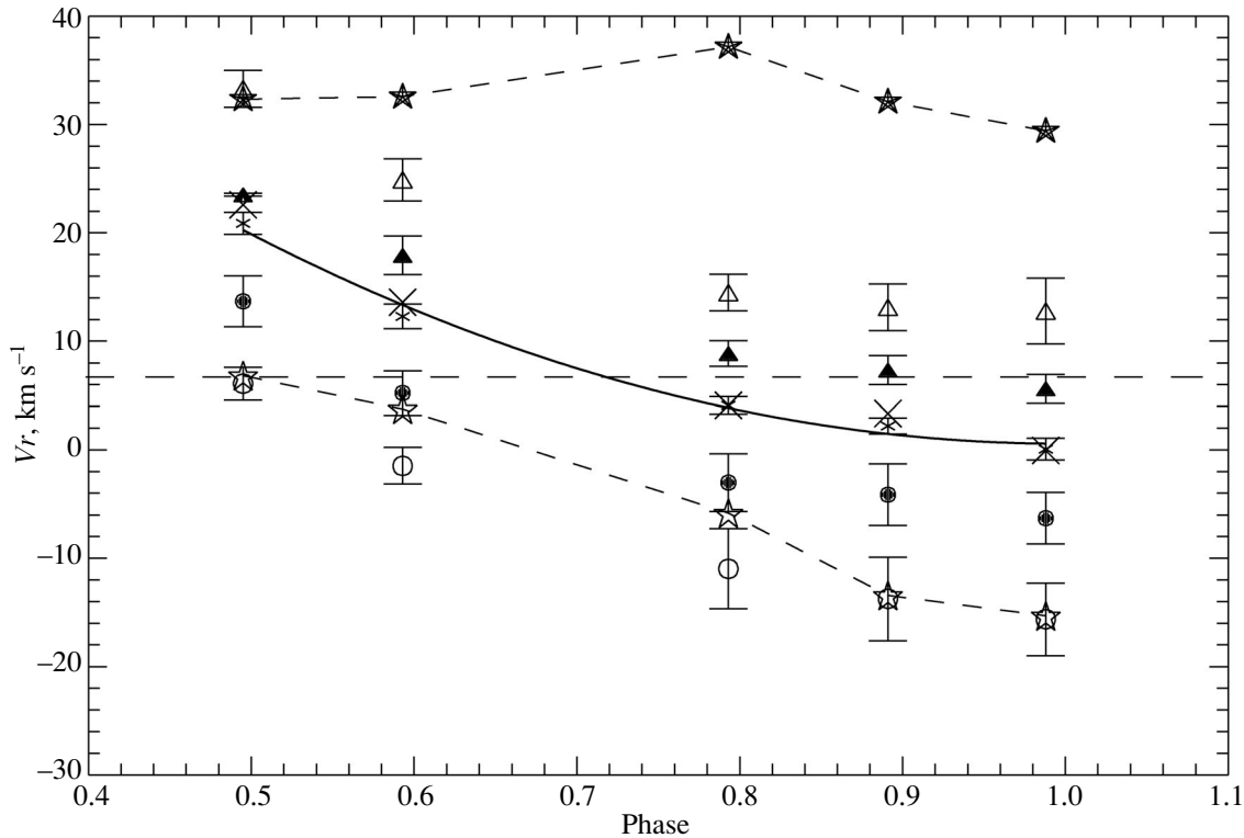
Fig. 9. Averaged estimates of the radial velocity V_r , measured from the cores of the metal absorption lines, their blue (B1, B2) and red (R1, R2) components, the H\alpha line, and its B and R components versus pulsation phase. The designations are the same as those in Fig. 8.
