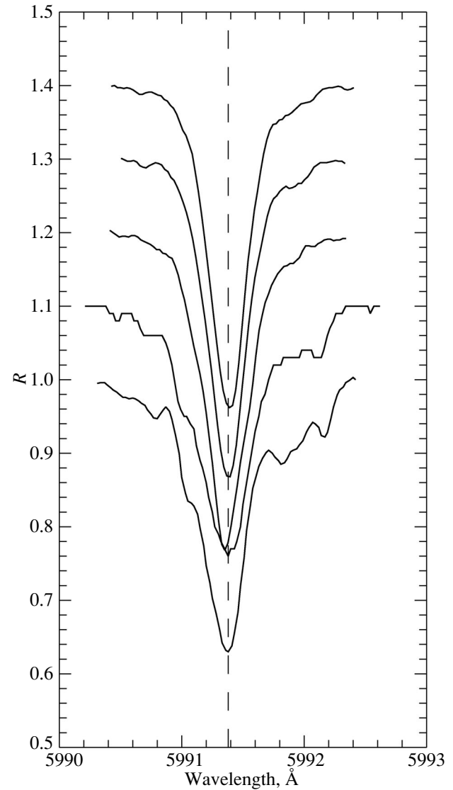
Fig. 2. Changes of the Fe II 5991.375 Å ( \chi_{\text{low}} = 3.15 eV) absorption line profile with increasing pulsation phase (from bottom to top).
