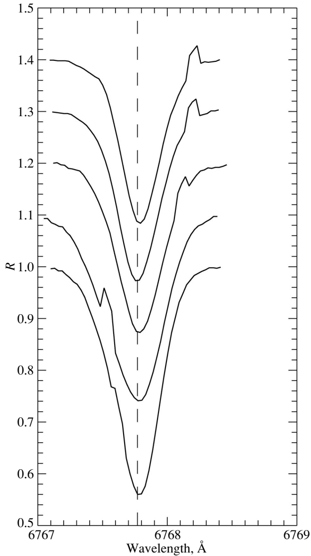
Fig. 1. Changes of the Cr I 6767.770 Å ( \chi_{\text{low}} = 1.83 eV) absorption line profile with increasing pulsation phase (from bottom to top).
