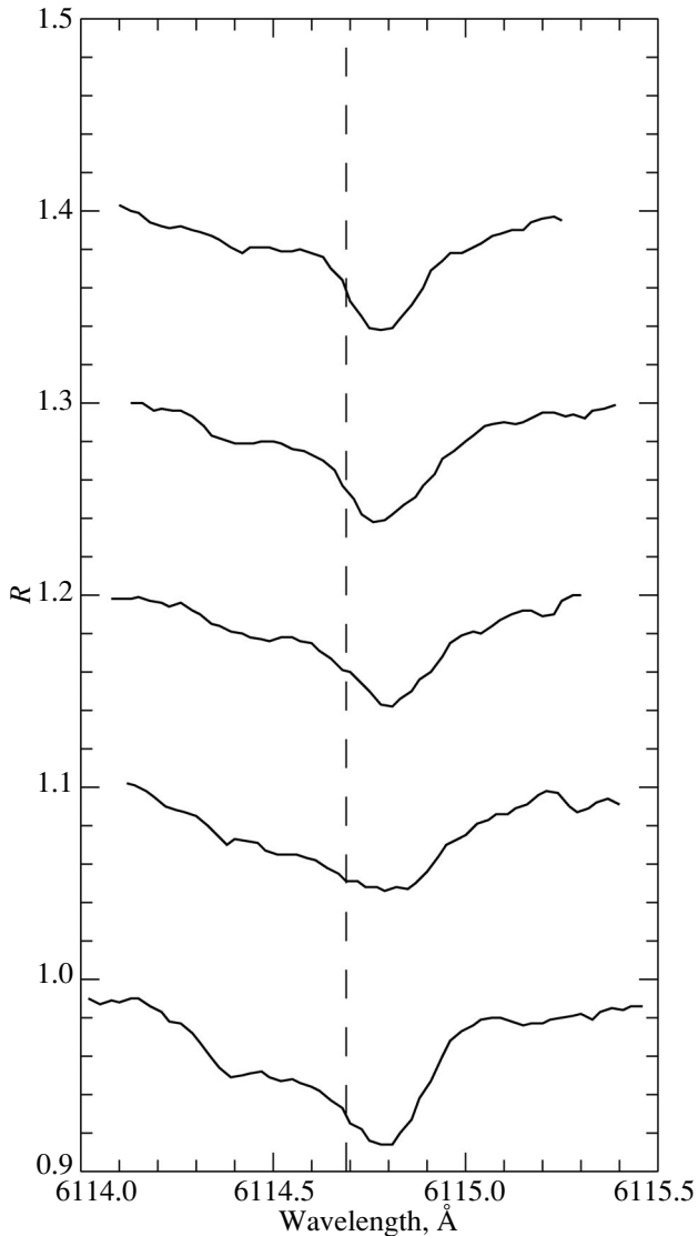
Fig. 5. Changes of the Zr II 6114.690 Å ( \chi_{\text{low}} = 1.66 eV) absorption line profile with increasing pulsation phase (from bottom to top).
