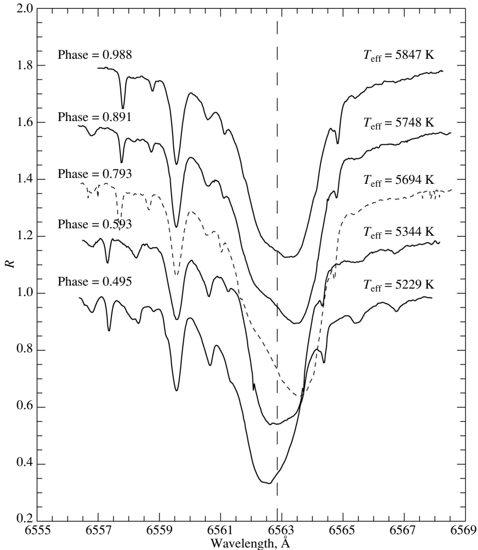
Fig. 7. Changes of the H \alpha 6562.850 Å absorption line profile with increasing pulsation phase.
