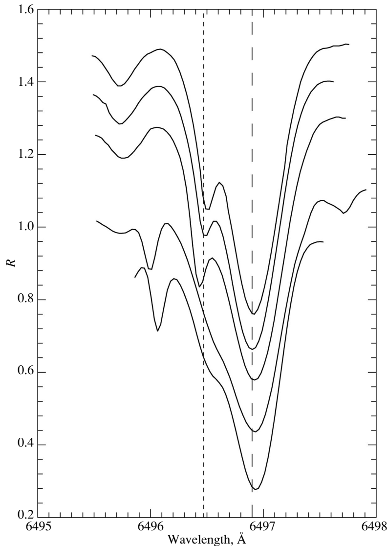
Fig. 3. Changes of the Ba II 6496.910 Å ( \chi_{\text{low}} = 0.60 eV) absorption line profile with increasing pulsation phase (from bottom to top).
