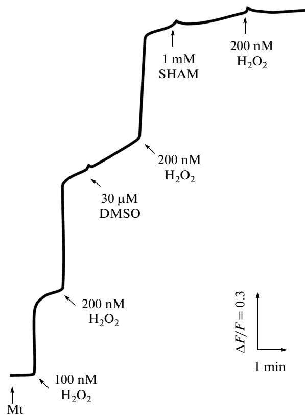
Fig. 2. Dependence of resorufin fluorescence on the H_2O_2 concentration in reaction medium in the presence of wheat mitochondria (Mt), and the effect of 1 mM SHAM on the signal. SHAM and its solvent DMSO were added in equivalent amount (2 \mu L/mL). Other conditions are described in the Materials and Methods section.
