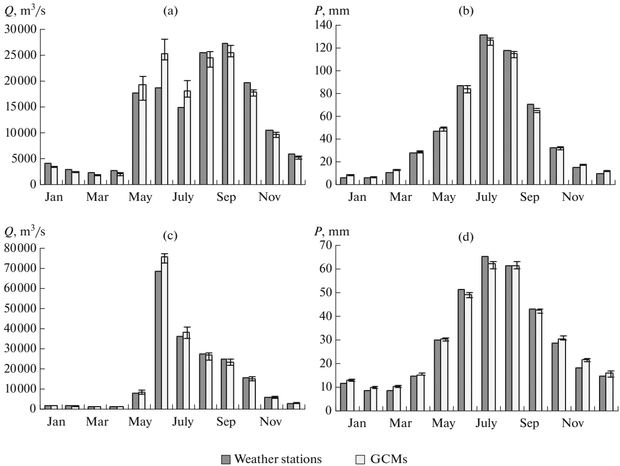
Fig. 3. Long-term average seasonal variations of river runoff and basin area-averaged precipitation, constructed by observational data and the average over the ensemble of climate models with the specification of the range of estimates by different GCMs over historical period 1970–1999 (the Amur R. (a, b), the Lena R. (c, d)).
