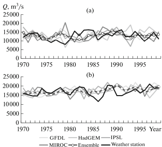
Fig. 4. Time variations of the annual runoff of (a) the Amur R. and (b) the Lena R., calculated by weather station data and data of an ensemble of climate models over the historical period.
