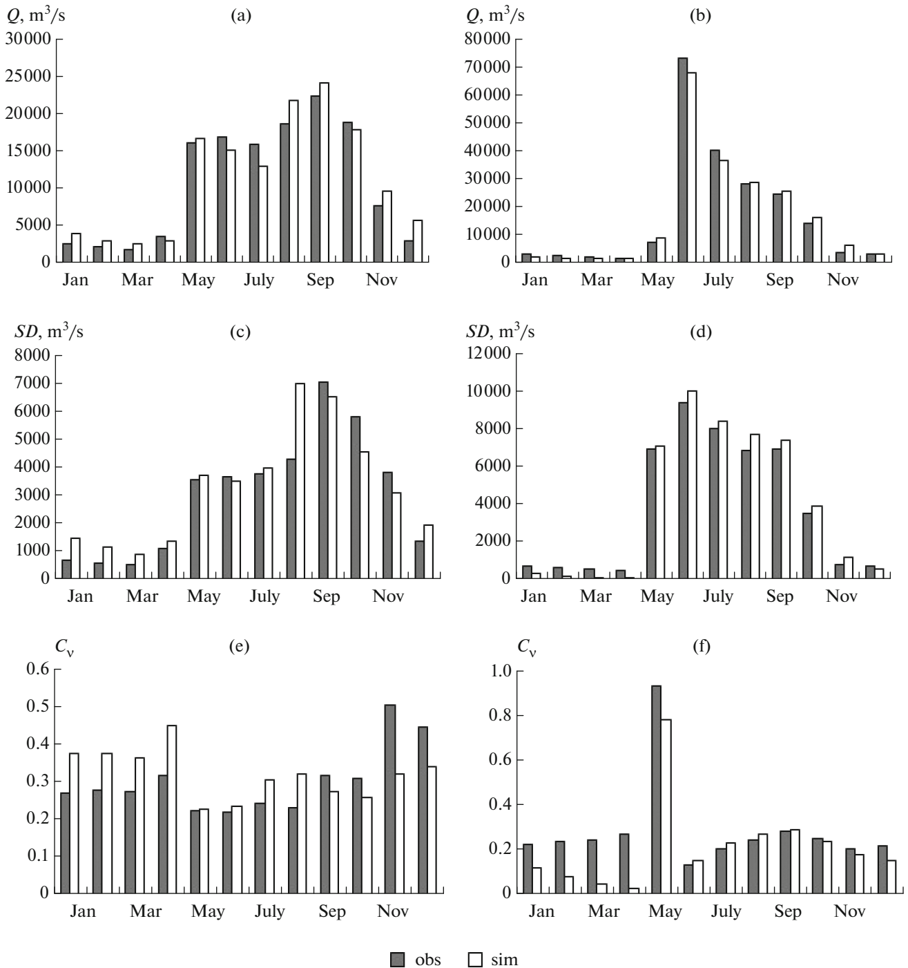
Fig. 2. Characteristics derived from the developed hydrological models of the Amur and Lena basins (1970–1999), including the long-term average, standard deviation, and the coefficient of variation of the mean monthly runoff at near-mouth gages: (a, c, e) for the Amur R. and (b, d, f) for the Lena R.
