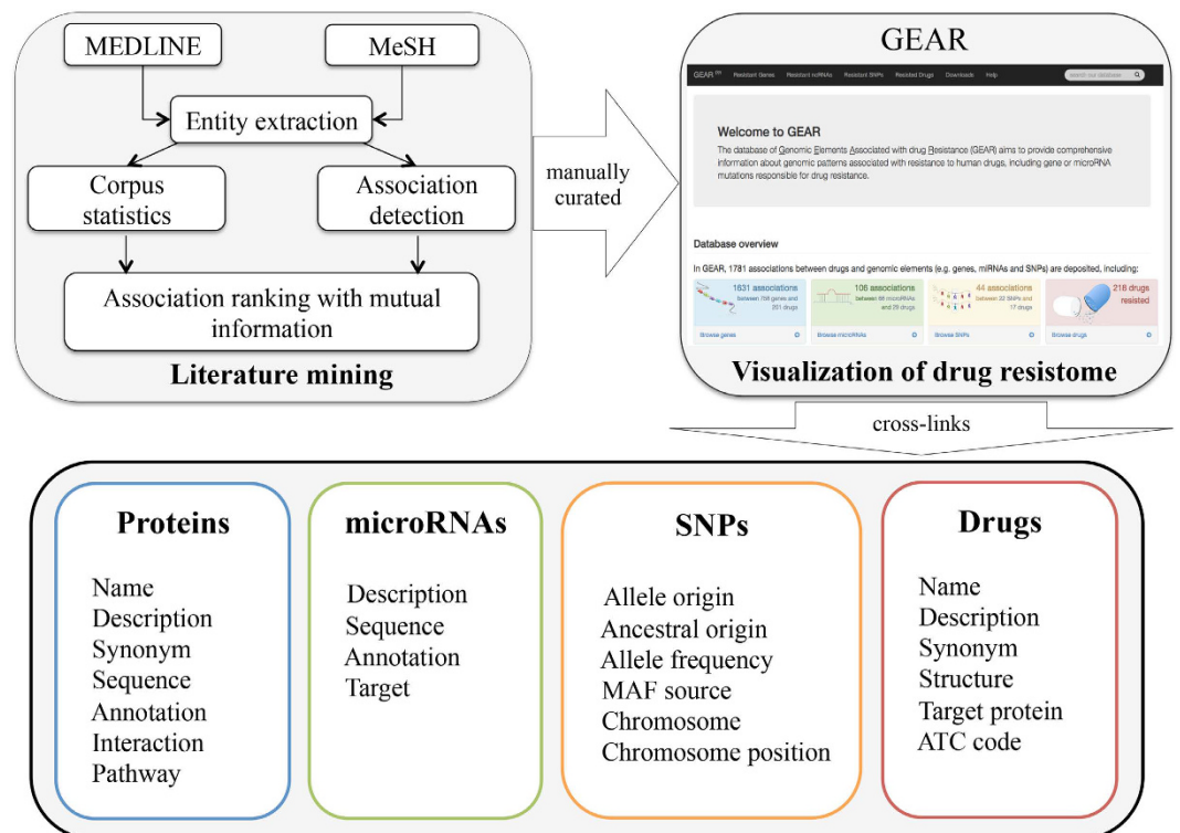
Figure 1. Schematic content of GEAR.
