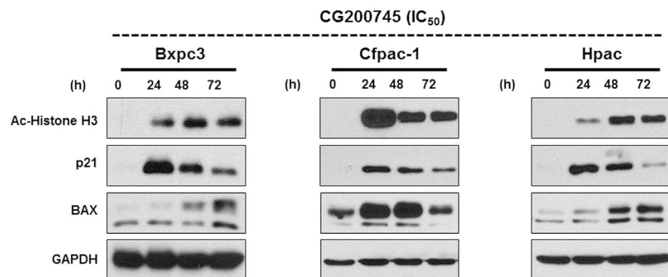
Figure 1. Anti-proliferative and pro-apoptotic activities of CG200745 against pancreatic cancer cells.
