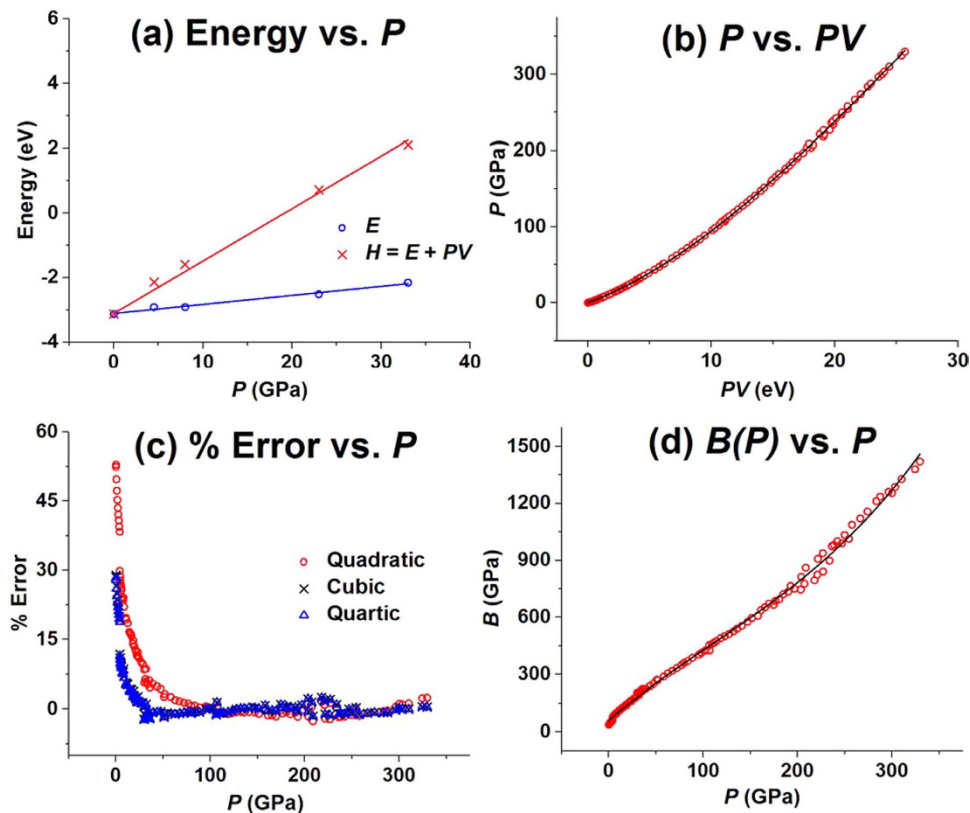
Figure 1. (a) The E -vs- P and H -vs- P plots calculated for Te, where E , H and PV are in eV units. The fitting coefficients a_1 , a_0 and b_1 for the linear plots E = a_1P + a_0 and H = b_1P + a_0 are respectively -3.0238 , 0.0246 and 0.1589 . (b) The P -vs- PV plot constructed from the experimental P -vs- V data for Te, where the solid line is the fitting curve obtained by using the cubic approximation for the EOS, Eq. 1. (c) The pressure-dependence of the % error, 100 \times (P_{\text{calc}} - P_{\text{expt}})/P_{\text{expt}} , of the P -vs- PV plot obtained for Te by using the cubic approximation of the EOS, Eq. 1. (d) The pressure dependence of the bulk modulus B(P) calculated for Te.
