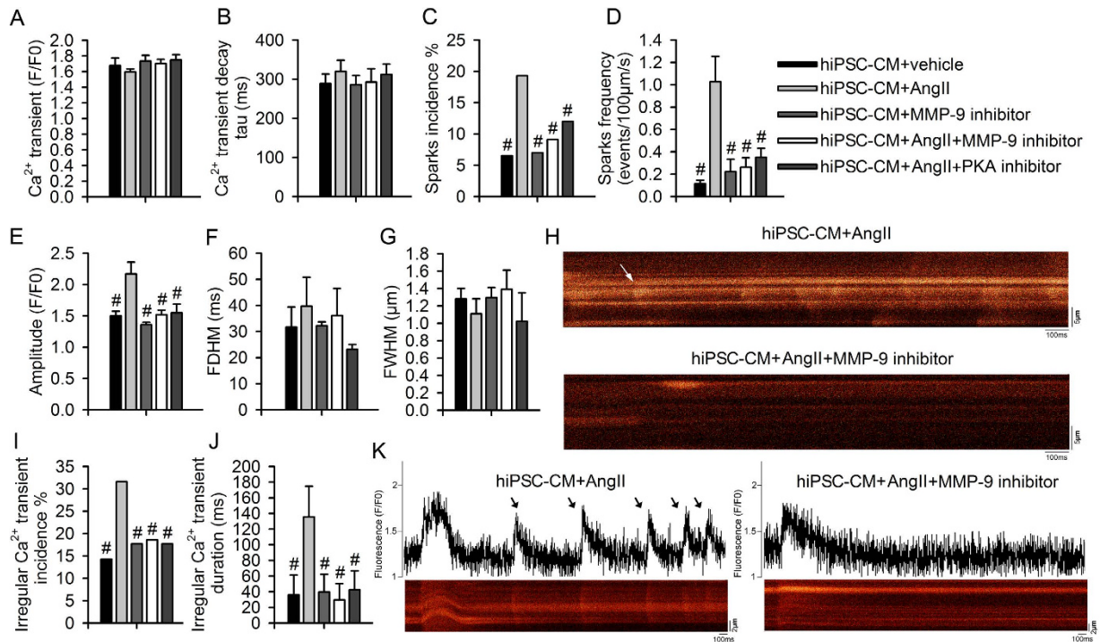
Figure 5. MMP-9 inhibition prevented Ca 2+ leakage and irregular calcium transients in hiPSC-CMs. (A and B) Amplitude and decay of Ca 2+ transients over time (n = 28–40, from 4 experiments, P = 0.48). (C to H) Summary of Ca 2+ spark, including the incidence (C), frequency (D), amplitude (E), duration (FDHM, F), and width (FWHM, G), as well as a representative image (H). Ca 2+ sparks (denoted by white arrows) after treatment with Ang II are prevented by an MMP-9 inhibitor (n = 50–145, from 6 to 8 experiments, # P < 0.05 vs. WT + Ang II). (I to K) A summary of irregular Ca 2+ transients, including their incidence (I) and duration (J), and a representative image (K). Irregular, arrhythmia-like calcium transients, denoted by black arrows, were induced only in a high-Ca 2+ (3.6 mM) Tyrode solution. Irregular, arrhythmia-like calcium transients, denoted by black arrows, were induced after treatment with Ang II and were prevented by MMP-9 or PKA inhibition (n = 33–73, from 3 to 5 experiments, # P < 0.05 vs. WT + Ang II). Data are shown as the mean ± SEM.
