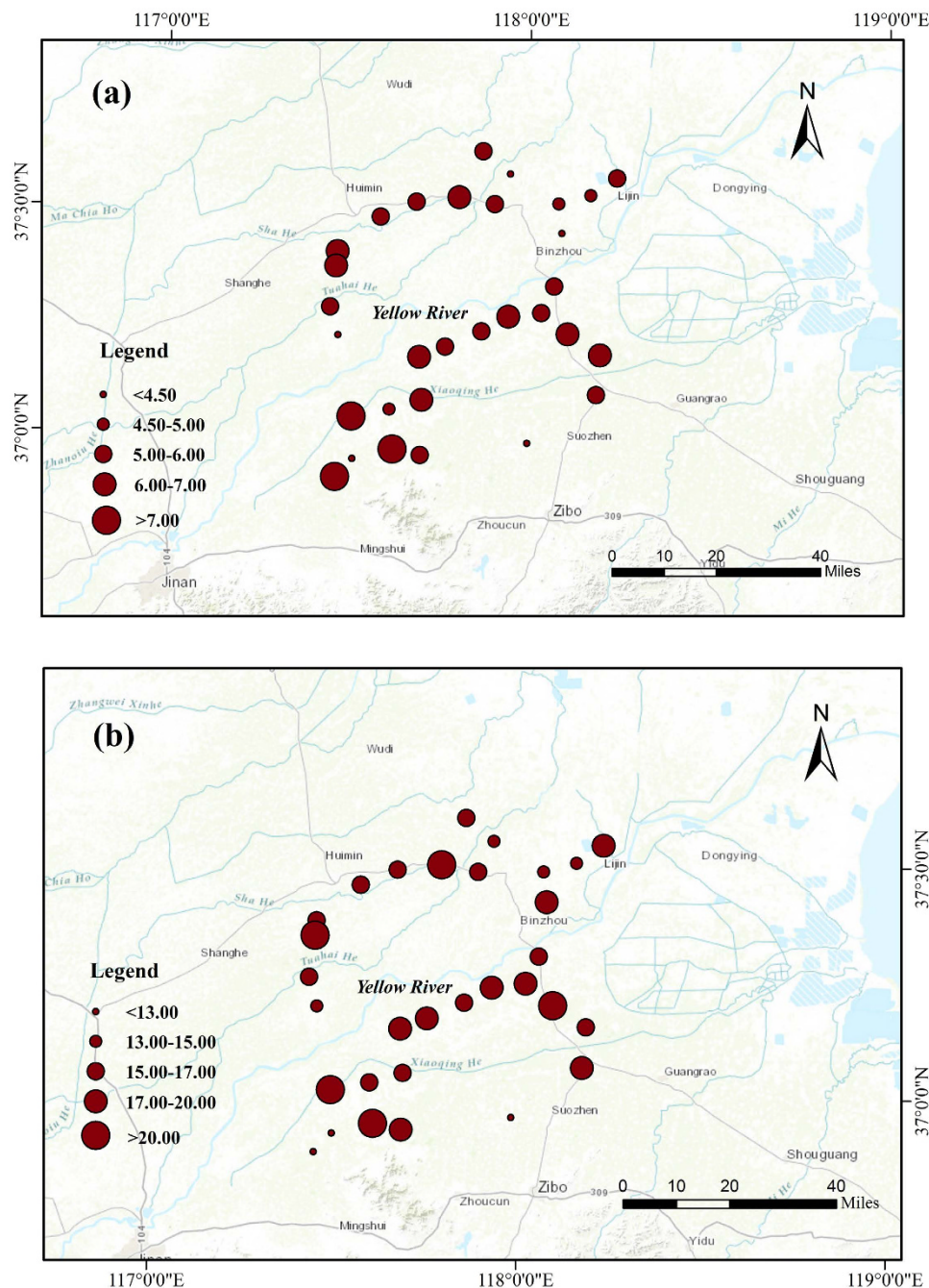
Figure 4. Spatial distributions of soil organic carbon (SOC) (a) and inorganic carbon (SIC) (b) stocks ( \text{kg C m}^{-2} ) over the 0–100 cm. The figure was generated by using ArcMap 10.1 ( http://www.esri.com/ ).
