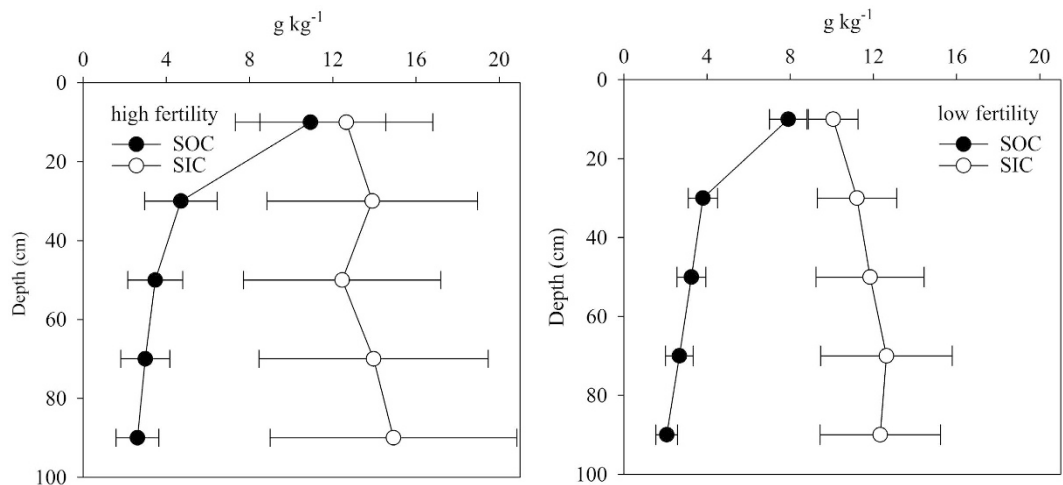
Figure 6. Vertical distributions of mean soil organic carbon (SOC) and inorganic carbon (SIC) for the high fertility (left) and low fertility (right) soils. The error bars indicate standard deviation. Soil profiles with \text{SOC} \geq 9 \text{ g kg}^{-1} in the upper 20 cm were regarded as high fertility, and profiles with \text{SOC} < 9 \text{ g kg}^{-1} were regarded as low fertility.
