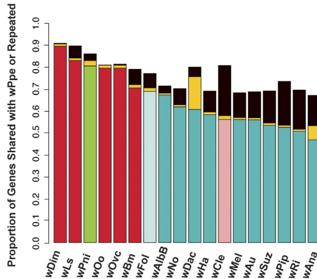
Figure 7. Gene repertoire similarity between several Wolbachia strains and Wolbachia from Pratylenchus penetrans (wPpe). For example, in strain wDim from Dirofilaria immitis , 90% of its genes have an ortholog in wPpe, whereas for strain wAna in Drosophila ananassae , 45% of its genes have orthologs in wPpe. Color scheme matches that in Fig. 4, except here yellow represents repetitive elements with orthologs in wPpe, and black indicates repetitive elements with no ortholog in wPpe.
