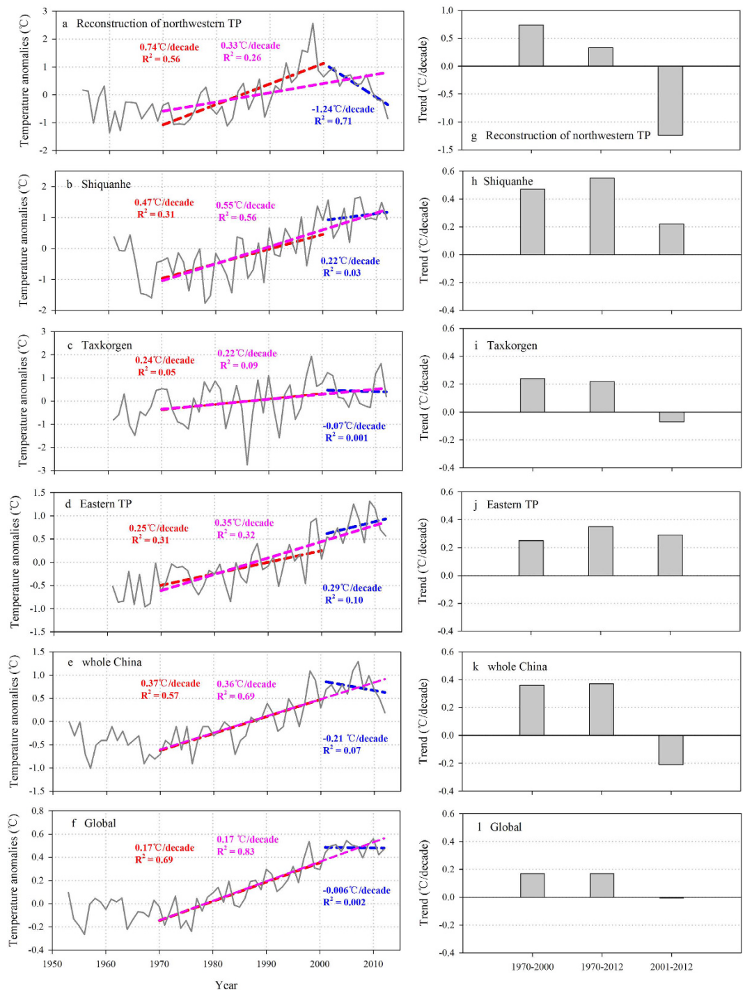
Figure 3. Linear trends of temperature series for the periods 1970–2000, 1970–2012 and 2001–2012. Figures on the left show the linear trends of the regional temperature reconstruction of the northwestern TP (a), the annual temperature series of Shiquanhe (b) and Taxkorgen (c) stations from the northwestern TP, temperature series based on all other stations from the eastern TP (d), as well as temperature series of China (e) and global temperature (f), for the periods 1970–2000 (red), 1970–2012 (pink) and 2001–2012 (blue) respectively. The color numbers represent linear trend values (°C/decade) and determination coefficients of the linear fits. Figures on the right (g–l) shows the bar charts of linear trends (°C/decade) for the three time periods corresponding to above temperature series.
