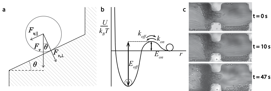
Figure 5. Schematic illustration of the angle-dependent viscous forces acting on a particle close to the wall (a) and the particle interaction potential with k_{on} and k_{off} the natural rate of agglomeration and detachment and E_{on} and E_{off} the corresponding energy barriers. (c) a zoomed-in, time series of a clog forming at a single constriction, with flow from left to right.
