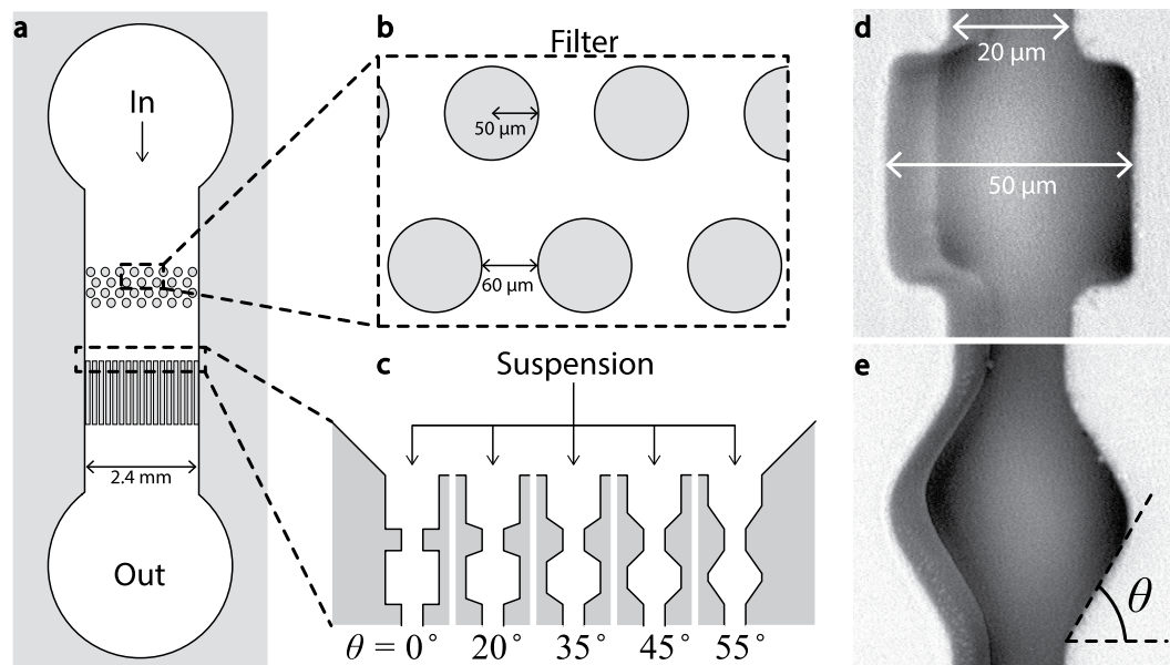
Figure 1. Overview of the multiplexed dead-end filtration micromodel: (a) an overview of the device geometry, (b) design of a pre-device filter which captures large contaminants such as dust or PDMS debris from the fluid, (c) a schematic illustration of the five different entrance angles studied. Each channel features a series of 19 constrictions with identical geometry along the flow direction. For statistics each channel type is repeated 6 times on each device; this allows 6-repeat measurements and 5 different geometries to be explored in a single experiment. (d) Scanning Electron Microscopy (SEM) picture of a \theta = 0^\circ constriction with its dimensions indicated and (e) a SEM picture of a \theta = 55^\circ constriction with the entrance pore angle \theta defined as indicated.
