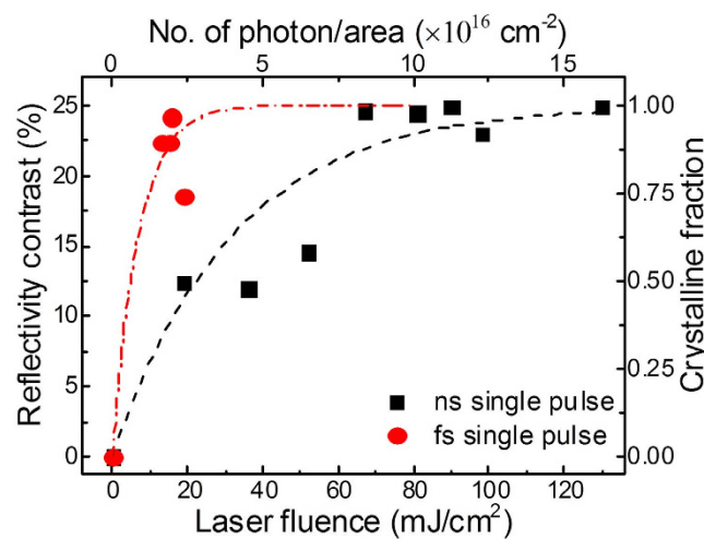
Figure 5. Optical reflectivity contrast of GST films at a wavelength of 650 nm after ns and fs laser pulse irradiation with a single pulse as a function of the laser fluence and the number of laser photons/area.
