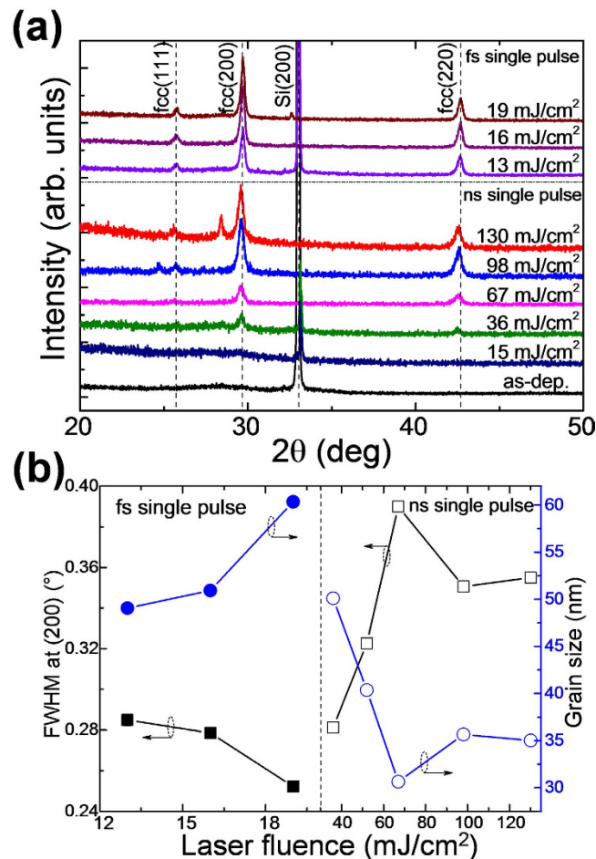
Figure 1. (a) XRD spectra of an as-deposited GST film and of films after 500 fs and 20 ns single laser pulse irradiation at different fluences. (b) FWHM of the rocksalt phase GST(200) reflection and corresponding calculated average grain sizes as a function of laser fluence (fs and ns denoted by the symbols with interior solid and open, respectively).
