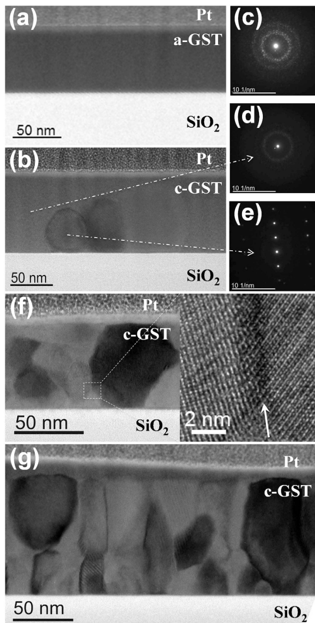
Figure 2. Cross-sectional BF-TEM images and NBD pattern of GST thin films: (a) and (c) as-deposited; (b,d,e) after ns laser pulse irradiation with 36 mJ/cm 2 ; (f) after ns laser pulse irradiation with 67 mJ/cm 2 , the insets show magnified regions; (g) after fs laser pulse irradiation with 19 mJ/cm 2 .
