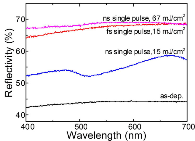
Figure 4. Optical reflectivity of GST films after deposition (as-dep.), after 20 ns single laser pulse irradiation at fluences of 15 and 67 mJ/cm 2 , and after 500 fs single laser pulse irradiation at a fluence of 15 mJ/cm 2 .
