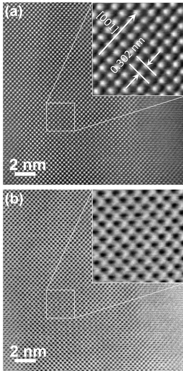
Figure 3. Aberration-corrected (a) MAADF- and (b) LAADF-HRSTEM images of a representative fs single laser pulse irradiated GST film viewed along the [001] zone axis. The insets show a magnification of the marked region. The corresponding overview image is shown in the Supplementary Section 2 (Fig. S2).
