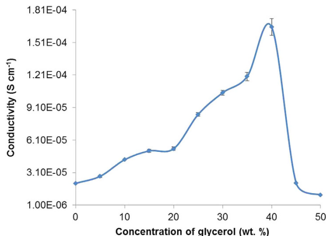
Figure 1. The conductivity of CMC-OA-Gly SBES at room temperature.
