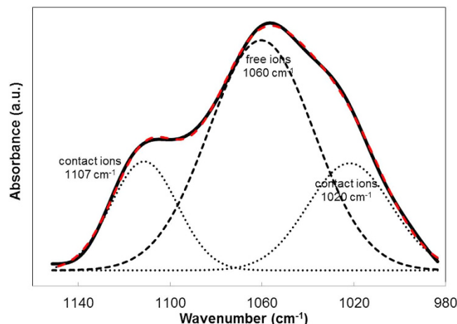
Figure 2. FTIR deconvolution of Gly-40.
