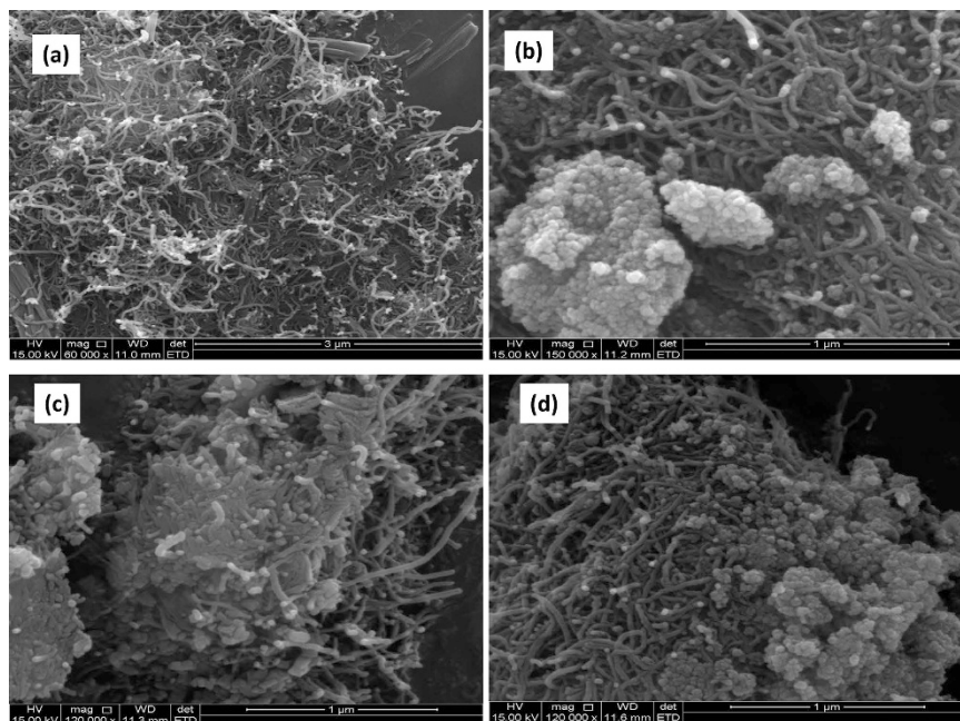
Figure 4. SEM images of (a) MWCNT/ \text{ZnO} /2,3-Nc, (b) MWCNT/ \text{Fe}_3\text{O}_4 /2,3-Nc (c) MWCNT \text{ZnO} /29H,31H-Pc and (d) MWCNT/ \text{Fe}_3\text{O}_4 /29H,31H-Pc.
