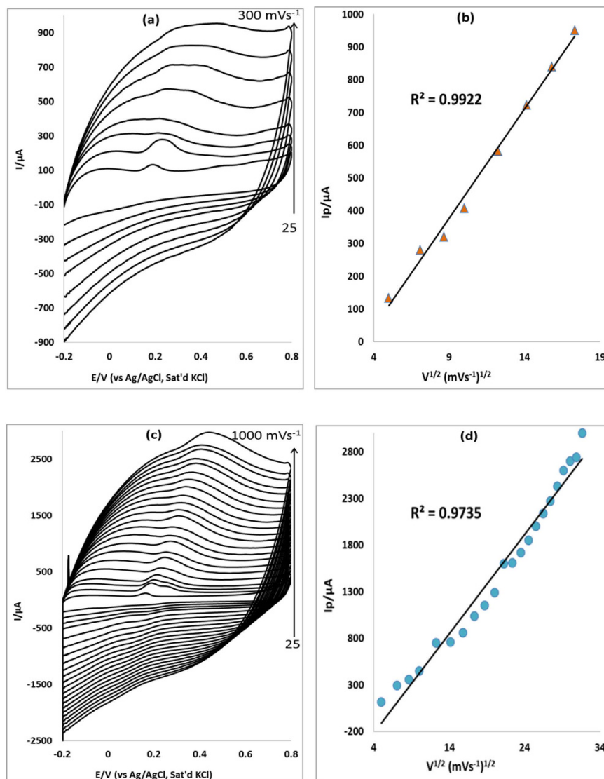
Figure 9. Cyclic voltammograms of (a) MWCNT/Fe 3 O 4 /2,3-Nc and (c) MWCNT/Fe 3 O 4 /29H,31H-Pc modified electrodes at scan rate (range 25–300 \text{mVs}^{-1} ) and (range 25–1000 \text{mVs}^{-1} ) respectively in pH 7.2 PBS containing 0.14 mM of EP. (b,d) are peak current vs. square root of scan rate plots of MWCNT/Fe 3 O 4 /2,3-Nc and MWCNT/Fe 3 O 4 /29H,31H-Pc electrodes respectively.
