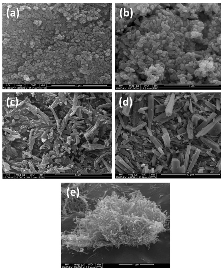
Figure 3. SEM images of (a) \text{Fe}_3\text{O}_4 , (b) \text{ZnO} , (c) 2,3-Nc, (d) 29H,31H-Pc, (e) MWCNT.
