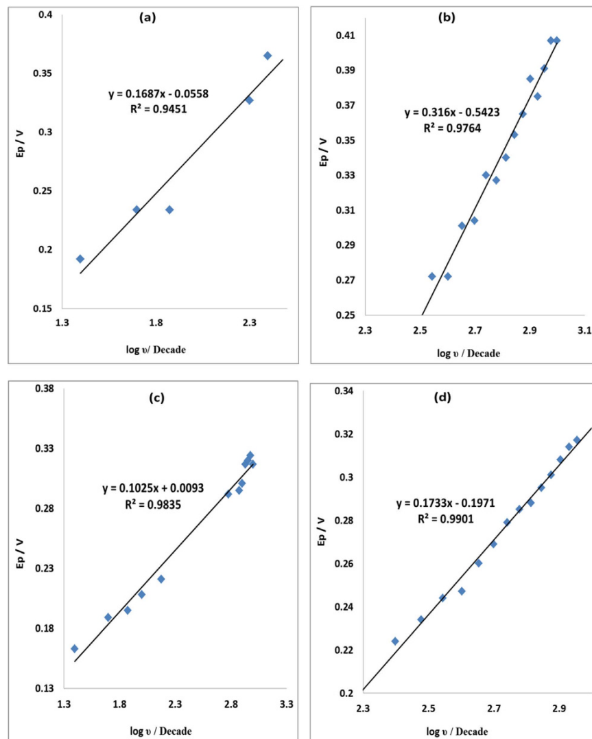
Figure 11. Plots of peak potential ( E_p ) versus \log v of (a) MWCNT/Fe 3 O 4 /2,3-Nc, (b) MWCNT/Fe 3 O 4 /29H,31H-Pc (c) MWCNT/ZnO/2,3-Nc and (d) MWCNT/ZnO/29H,31H-Pc in pH 7.2 PBS containing 0.14 mM of EP.
