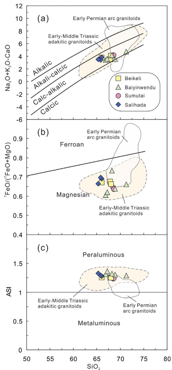
Figure 4. Selected major element diagrams for the Beikeli, Baiyinwendu, Sumutai and Salihada plutons. (a) \text{Na}_2\text{O} + \text{K}_2\text{O} - \text{CaO} vs. \text{SiO}_2 diagram 56 , (b) \text{TFeO}/(\text{TFeO} + \text{MgO}) vs. \text{SiO}_2 diagram 56 and (c) ASI vs. \text{SiO}_2 diagram 56 . \text{TFeO} = \text{FeO} + 0.9 \text{Fe}_2\text{O}_3 , \text{ASI} = \text{molecular Al}/(\text{Ca} - 1.67\text{P} + \text{Na} + \text{K}) . Data for the early Permian arc granitoids and Early-Middle Triassic adakitic granitoids are from refs 15, 19 and 23.
