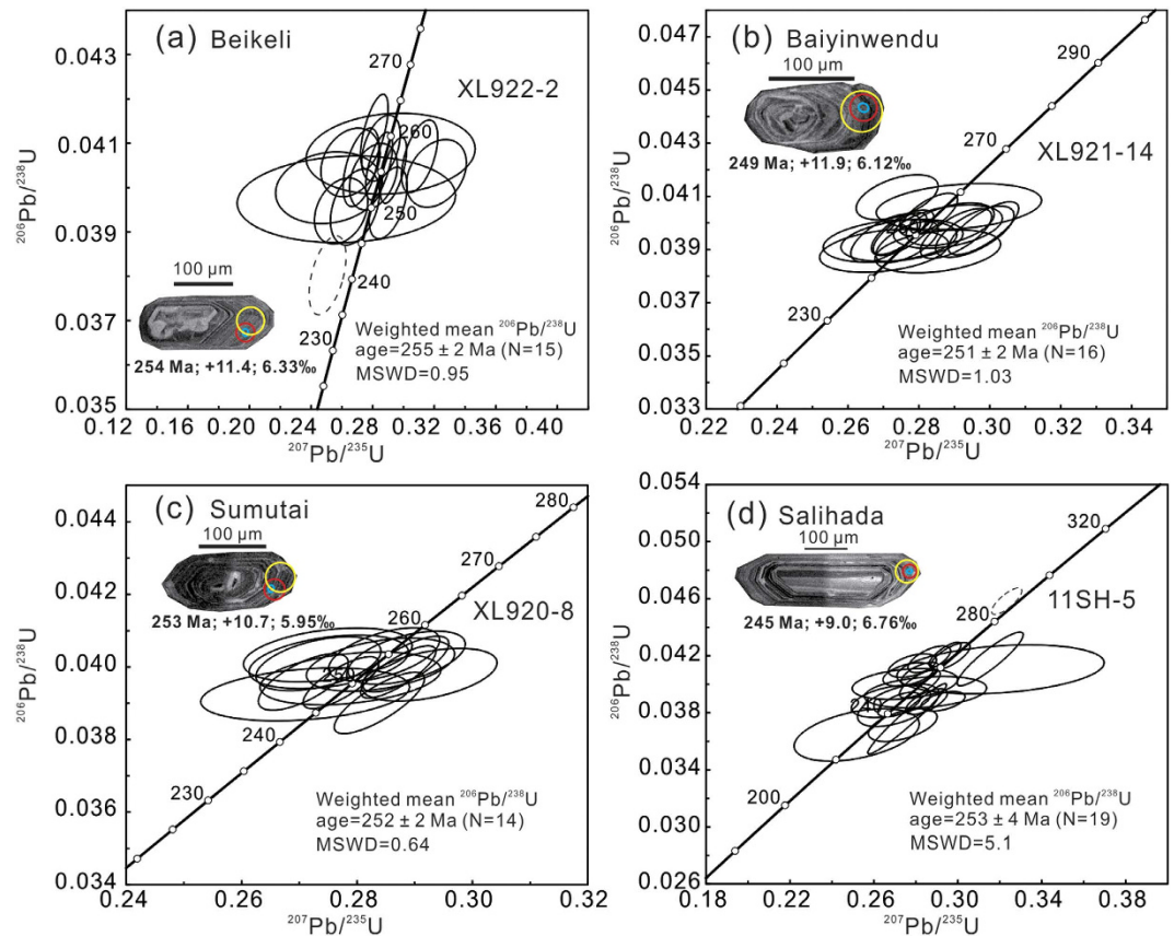
Figure 3. Cathodoluminescence (CL) images of selected zircon grains and U-Pb concordia diagrams. (a) Granodiorite (XL922-2) from the Beikeli pluton, (b) Granodiorite (XL921-14) from the Baiyinwendu pluton, (c) Granodiorite (XL920-8) from the Sumutai pluton, and (d) Granodiorite (11SH-5) from the Salihada pluton. Zircon U-Pb ages (red circles), \epsilon_{\text{Hf}}(t) values (yellow circles) and \delta^{18}\text{O} values (black circles).
