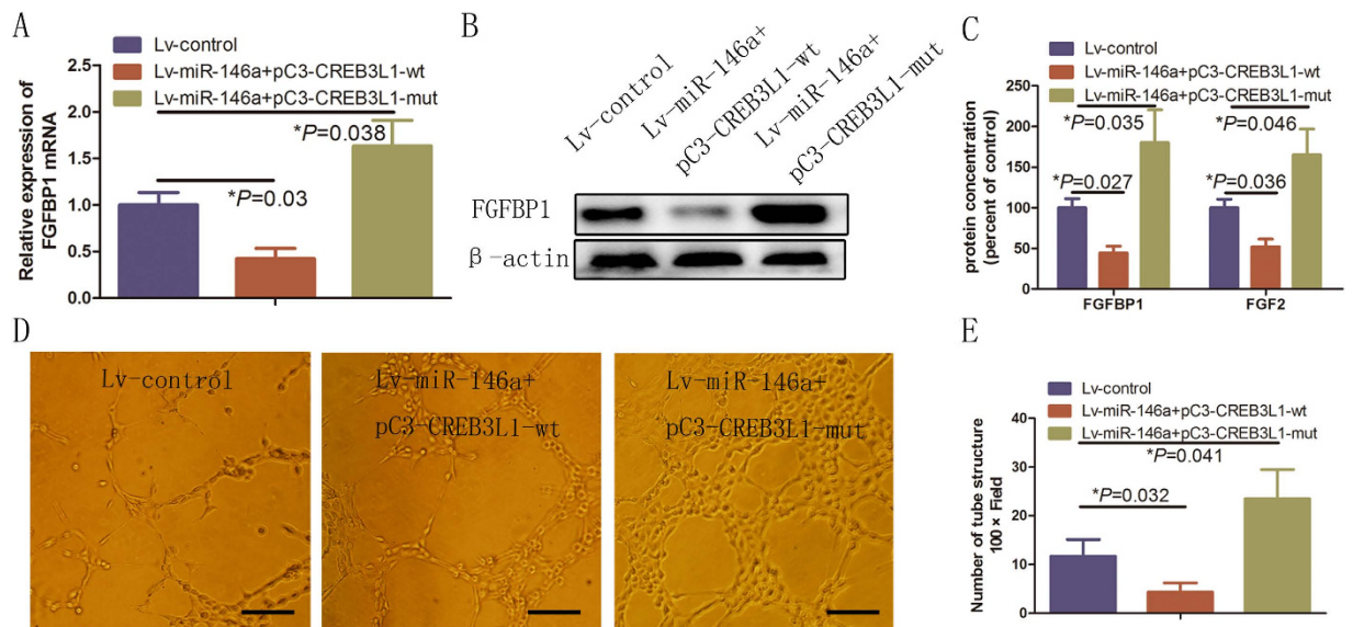
Figure 6. CREB3L1 was a mediator in miR-146a over expression-induced FGFBP1 and FGF2 expression.
