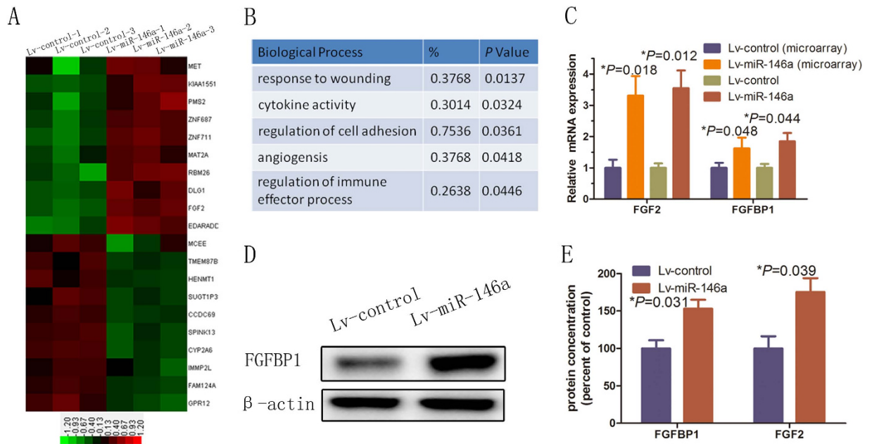
Figure 2. miR-146a promoted FGF2 and FGFBP1 expression. (A) Cluster analysis of mRNA expression profiles. Total RNA isolated from three biological replicates of Lv-miR-146a and Lv-control HUVECs was subjected to microarray analysis. The mRNA expression data were normalized to the average median of all genes present on the array. The mRNAs that were up-regulated at least 1.5-fold (red bars) or down regulated at least 2-fold (green bars) were considered for cluster analysis. (B) Gene Ontology classification of the predicted miR-146a target genes identified by integrating the results of four algorithms using the miRwalk website. (C) RT-qPCR was performed to determine FGF2 and FGFBP1 protein expression after infection of HUVECs with Lv-control or Lv-miR-146a. Error bars represent mean \pm SD from three experiments ( n = 3 ); *P < 0.05 . (D) Western blot analysis of FGFBP1. (E) ELISA analyses of FGFBP1 and FGF2 protein expression. Error bars represent mean \pm SD from three experiments ( n = 3 ); *P < 0.05 . ANOVA (C,E).
