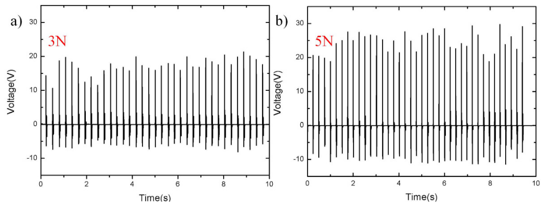
Figure 9. Output voltages of 2 wt% PDMS/MWCNT under different forces. (a) Output voltages of device under 3 N forces. (b) Output voltages of device under 5 N forces.
