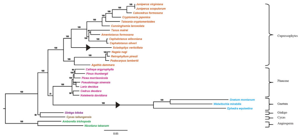
Figure 6. Maximum likelihood tree of 29 taxa from 59 plastid genes. Bootstrap values are shown along branches. Triangles on nodes indicate loss of accD from plastome.
