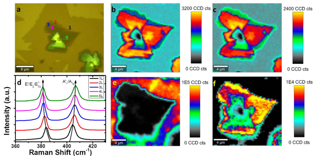
Figure 2. (a) Optical image of CVD MoS 2 with layer numbers labelled. (b) Peak intensity map of A 1 /A 1g (~403 cm -1 ) high-frequency Raman mode. (c) Peak intensity map of E g /E g 1 /E 2g 1 (~385 cm -1 ) Raman mode. (d) Raman spectra of 1–5L MoS 2 . (e) Peak intensity map of A 1 exciton PL peak. (f) Peak intensity map of B 1 exciton PL peak.
