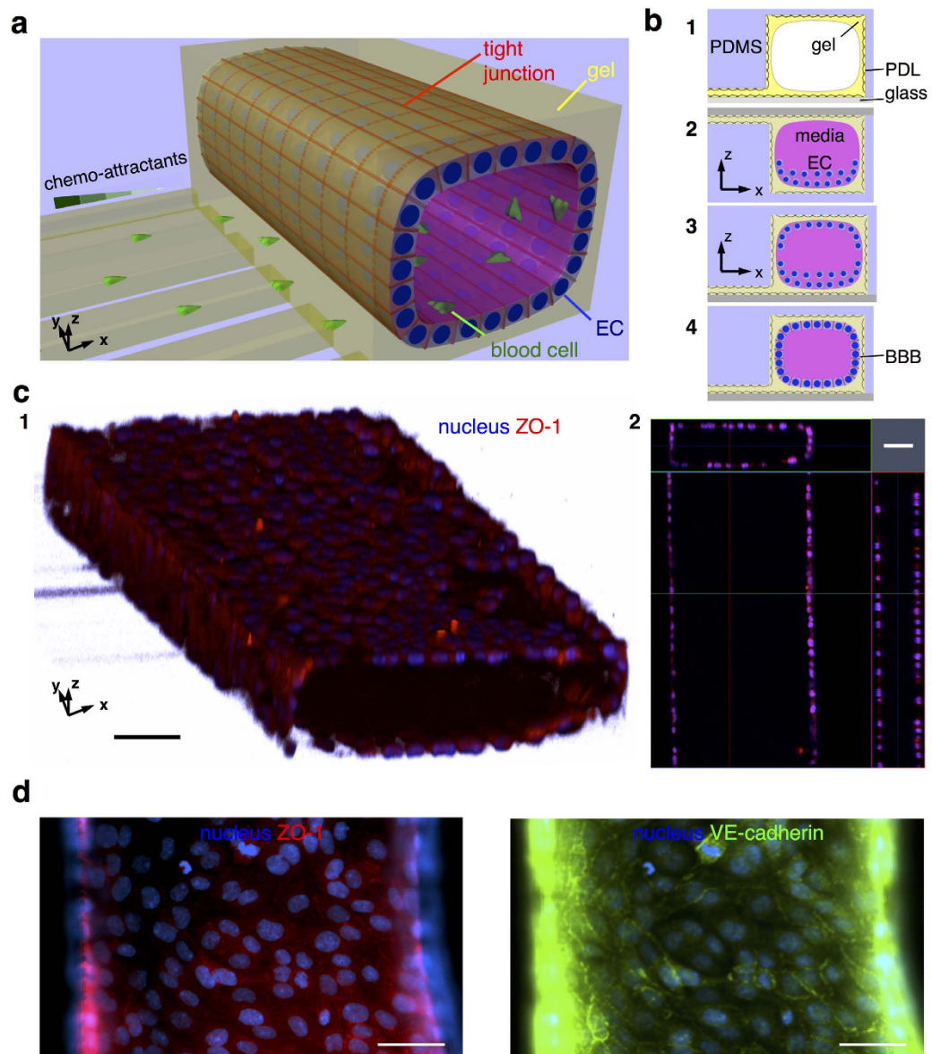
Figure 1. Schematic representation of a 3D in vitro BBB model and structural details. (a) A 3D BBB model consists of endothelial cells (EC) arranged in a cylindrical monolayer, forming a tight seal, and separating a “blood” compartment from an array of capillaries presenting chemotactic gradients, which simulate white blood-cell transmigration across the BBB. (b) The 3D BBB model is constructed by (1) coating an adhesive molecules, Poly-D-lysine (PDL), and a gel on polydimethyl-siloxane (PDMS) microstructures and a glass substrate, (2) plating brain endothelial cells (EC) first on the top and (3) later on the bottom surfaces, and (4) culturing to form tight monolayers. (c) The constructed BBB model has a lumen lined by confluent monolayers of endothelial cells on all surfaces, which resembles in vivo BBB. Prospective (1) and cross-sectional (2) views are presented. (d) The formation of a tight BBB is confirmed by the imaging of localized tight junction-involving proteins along cellular boundaries. Fluorescent Zonula Occluden-1 (ZO-1) and Ve-Cadherin proteins are shown in left and right panels, respectively. Scale bars, 50 \mu\text{m} .
