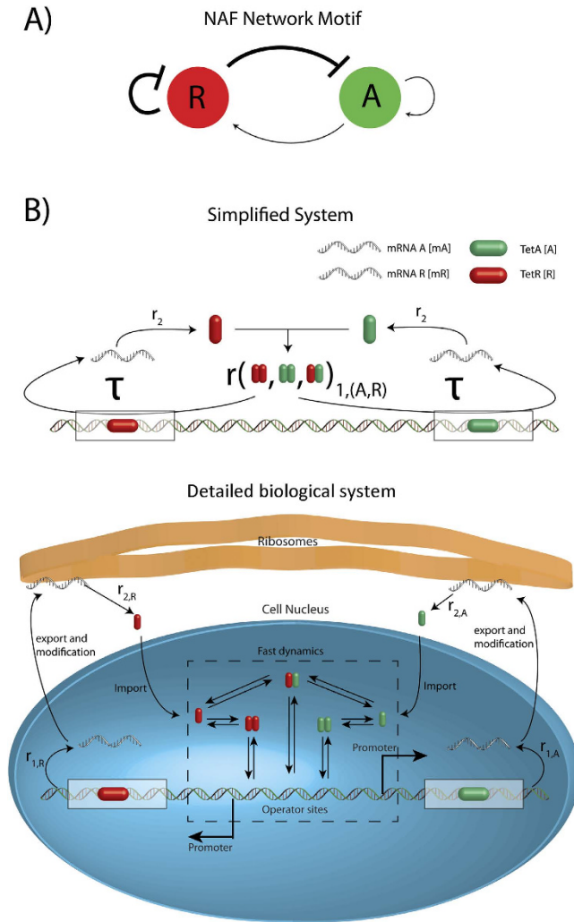
Figure 1. Schematic overview of the model. (A) The NAF motif consists of an autoregulated repressor coupled with an autoregulated activator. (B) Comparing the biologically realistic system where several steps are involved, we simplify the system as follows. Starting from the top left, mRNA at ribosomes are translated into proteins with rate r_2 , the import of proteins is very fast, and therefore it is neglected 19 . Second, the chemical reactions are fast and both dimerization and protein-DNA binding are therefore treated as being in an equilibrium 20 . The last step in the simple model is production of mRNA. This step covers transcription of mRNA, modification and export of mRNA from the nucleus to the ribosomes. The transcription rate is regulated by dimers (activator-activator, repressor-repressor, activator-repressor) binding to the operator sites and the modification and export of mRNA is simplified by a 30 minute time delay ( \tau ) 13,18 . The simplified system can be schematically represented by the NAF motif in (A). The equations governing the simplified system are described in the Materials and methods section.
