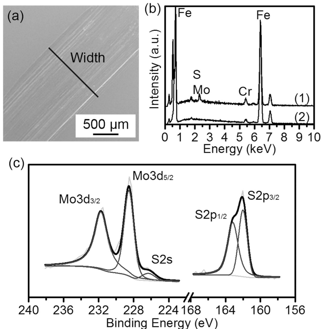
Figure 3. The analysis of the wear scar of the test of the lubricant containing the as-synthesized \text{MoS}_2 nanosheets stopped at 2000 N. (a) The SEM image of the wear scar and the width is about 1.39 \pm 0.06 mm. (b) The EDS spectra (1) inside and (2) outside the wear scar, and the elements of Mo and S can only be detected inside the wear scar. (c) XPS analysis of the elements of Mo and S in the wear scar, with \text{Mo}3d_{3/2} at 231.7 eV, \text{Mo}3d_{5/2} at 228.6 eV, \text{S}2s at 226.3 eV, \text{S}2p_{1/2} at 163.2 eV and \text{S}2p_{3/2} at 162.0 eV.
